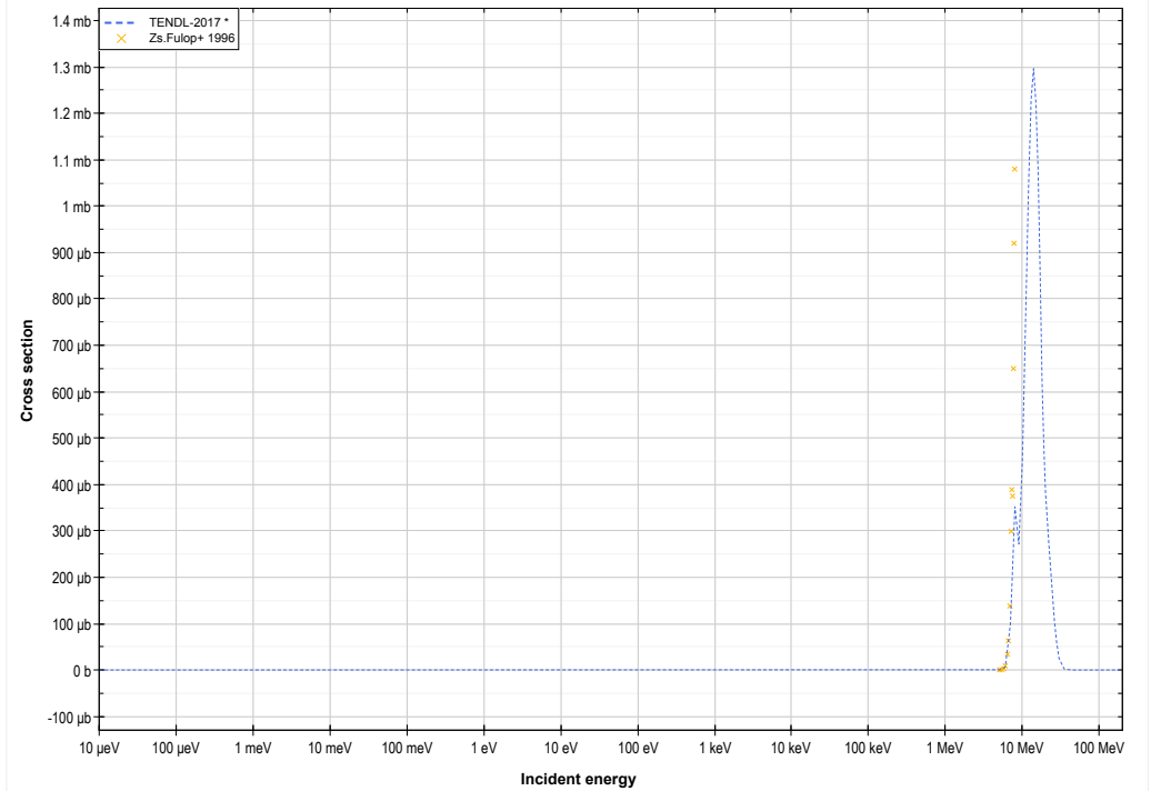
Ge70 ( \alpha, \gamma ) or Se74 production lin-log
