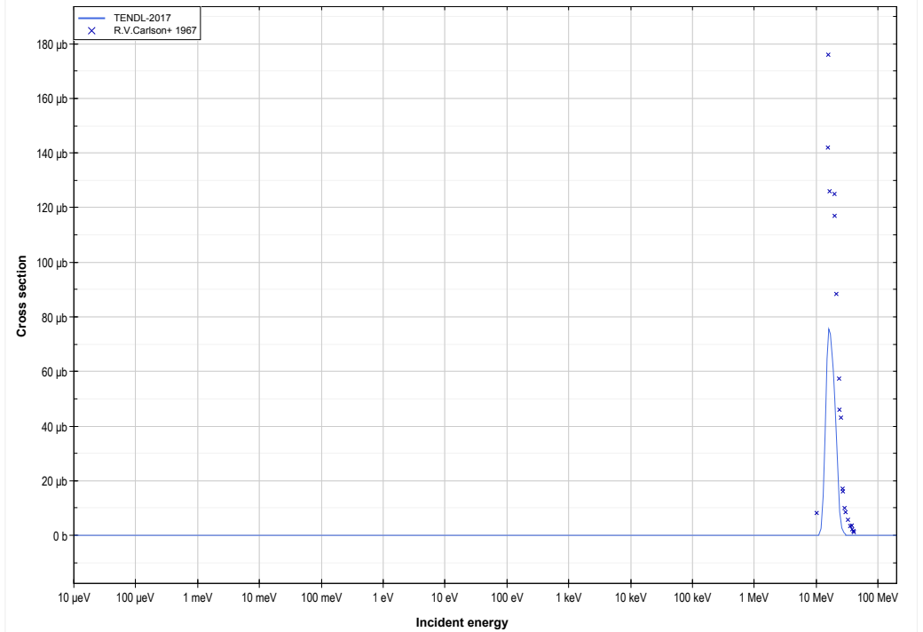
1127 ( \alpha,\gamma ) or Cs131 production lin-log
