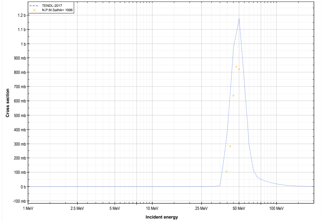
I127 ( \alpha,4n ) or Cs127 production lin-log
