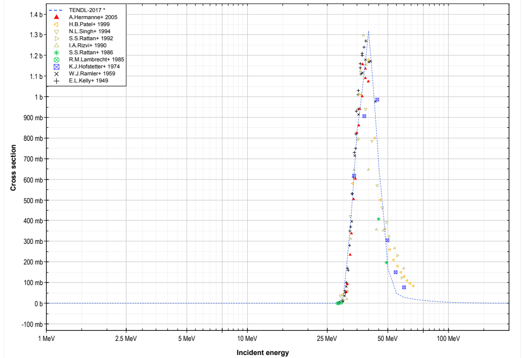
Bi209 ( \alpha,3n ) or At210 production lin-log
