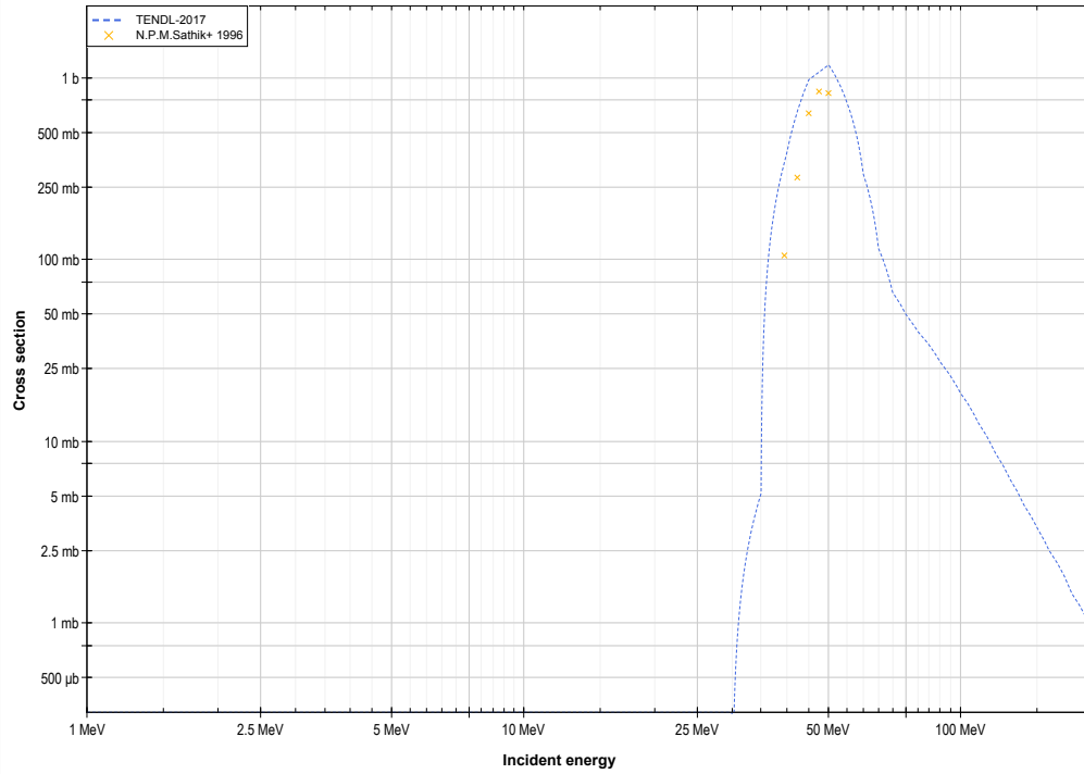
I127 ( \alpha,4n ) or Cs127 production log-log
