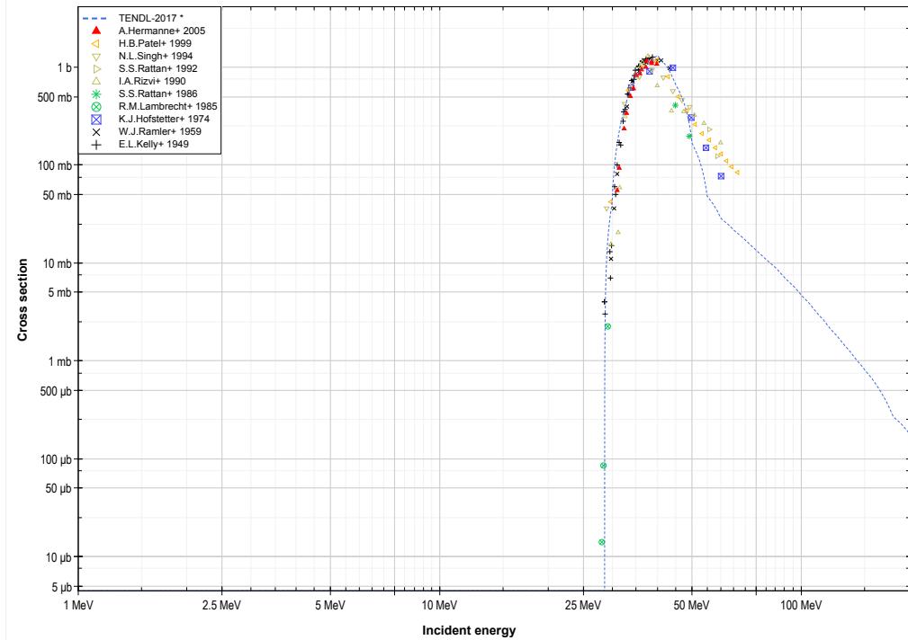
Bi209 ( \alpha,3n ) or At210 production log-log
