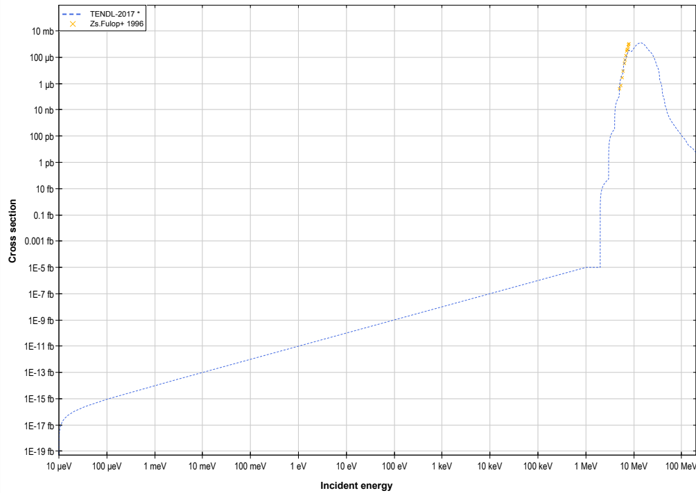
Ge70 ( \alpha, \gamma ) or Se74 production log-log
