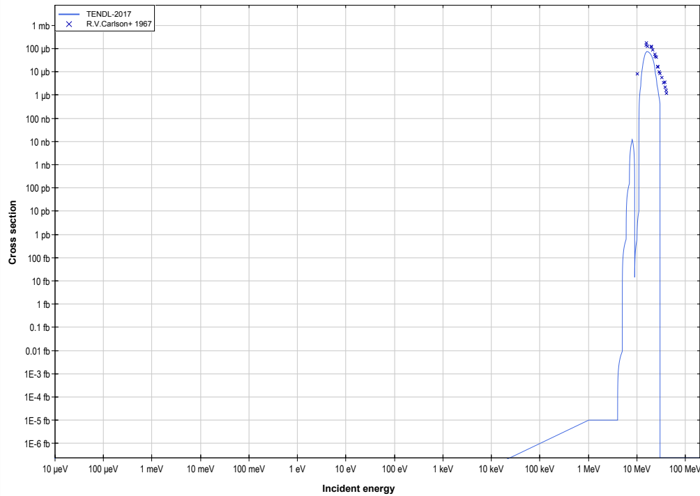
1127 ( \alpha,\gamma ) or Cs131 production log-log
