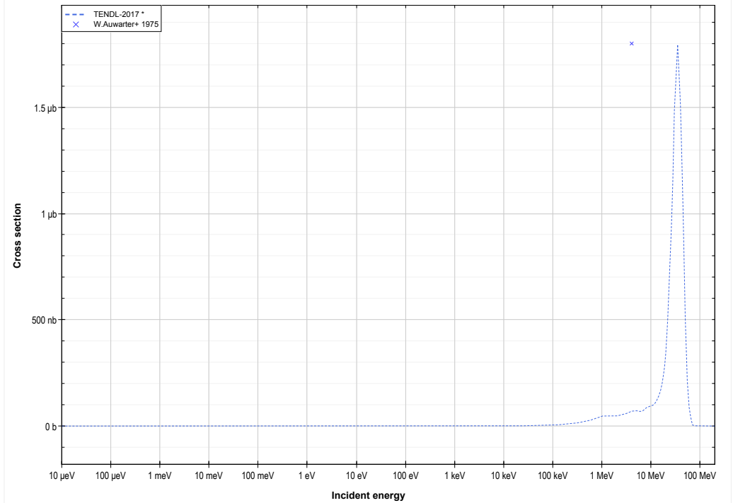
Li6 ( \alpha,\gamma ) or B10 production lin-log
