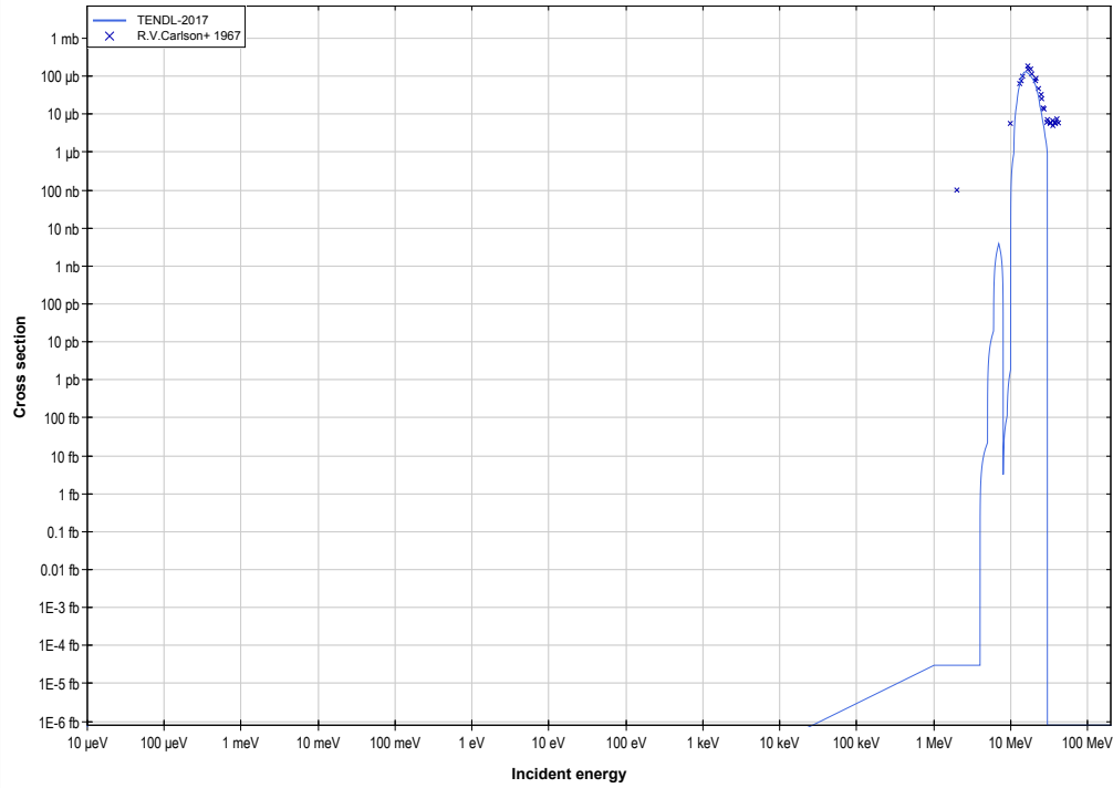
In115 ( \alpha,\gamma ) or Sb119 production log-log
