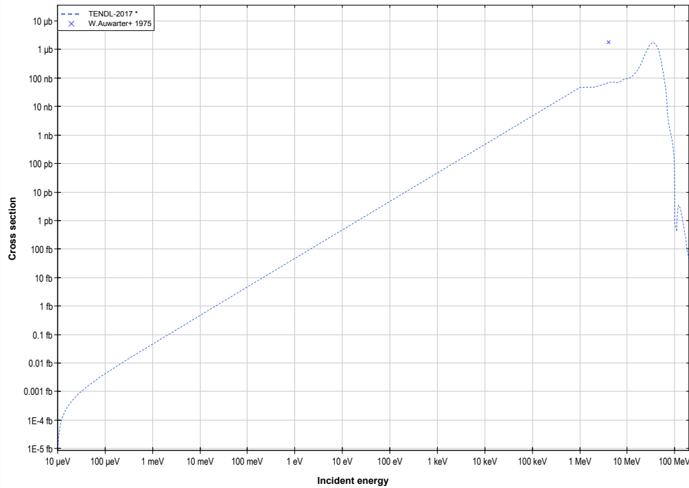
Li6 ( \alpha,\gamma ) or B10 production log-log
