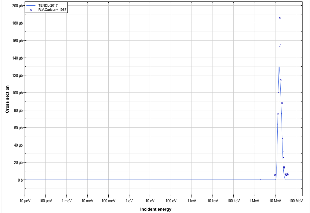
In115 ( \alpha,\gamma ) or Sb119 production lin-log
