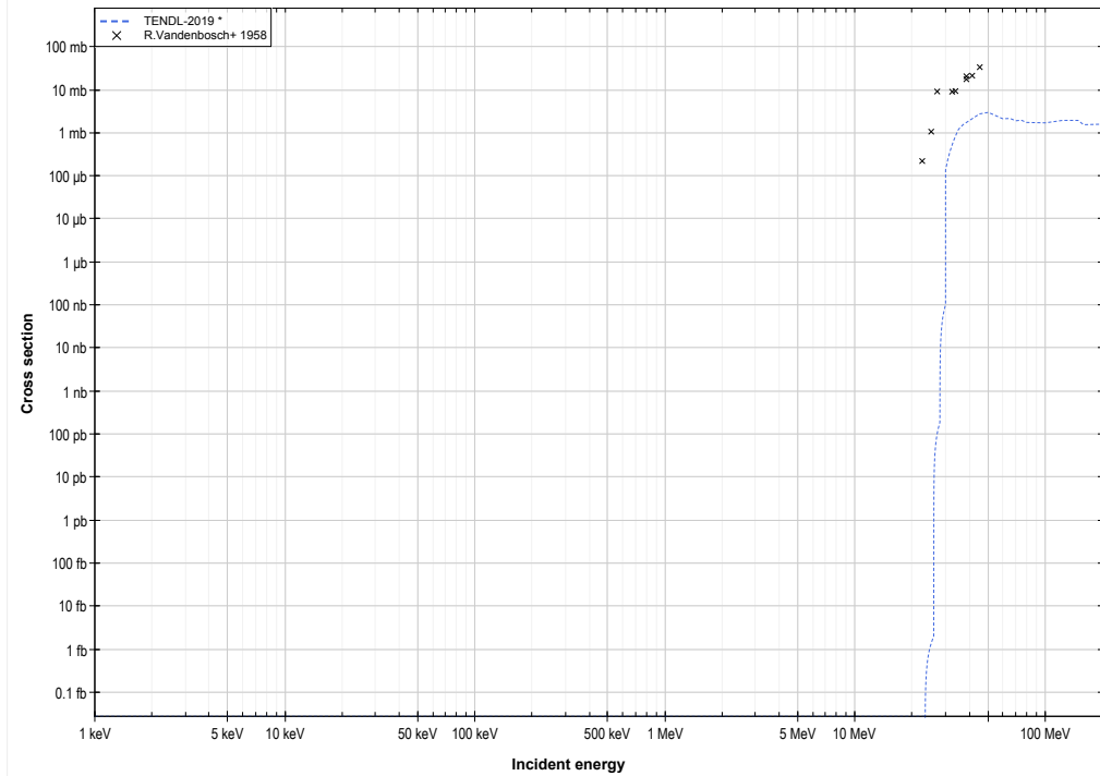
U238 ( \alpha,2n+p ) or Np239 production log-log
