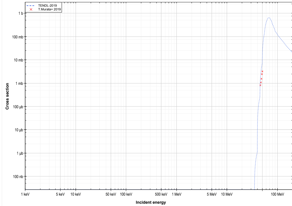
Y89 ( \alpha,4n+p ) or Zr88 production log-log
