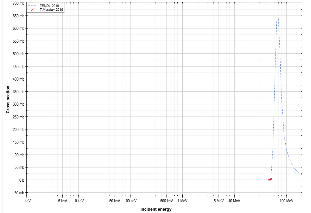
Y89 ( \alpha,4n+p ) or Zr88 production lin-log
