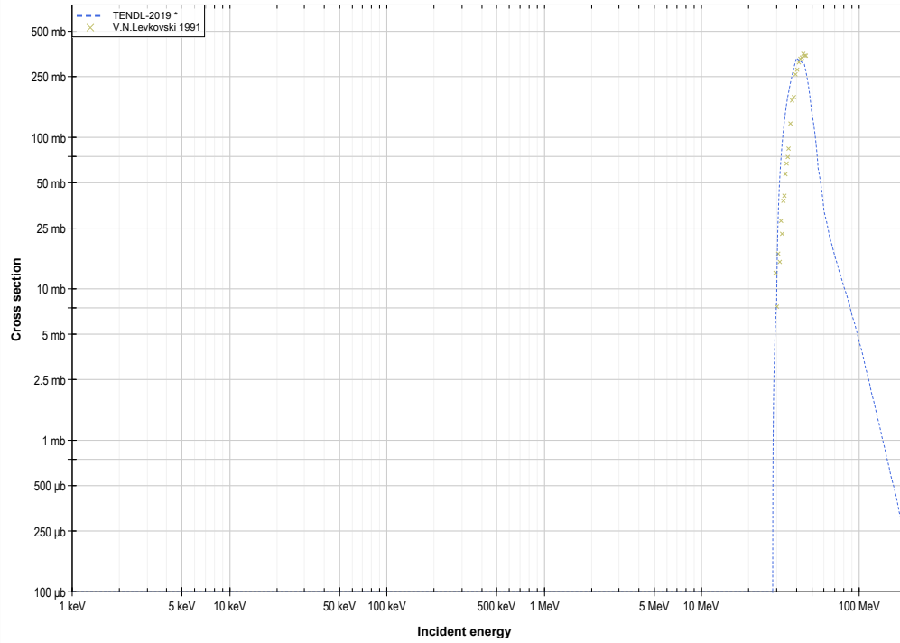
Se76 ( \alpha,3n ) or Kr77 production log-log
