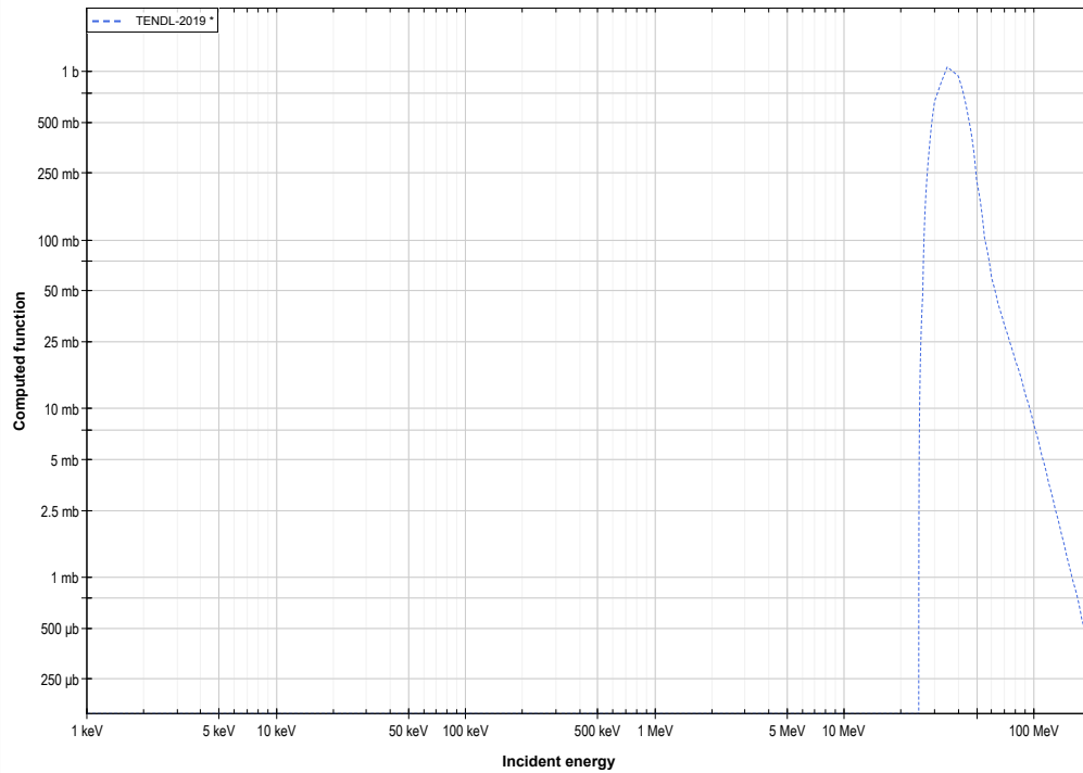
Br81 ( \alpha,3n ) or Rb82 production log-log
