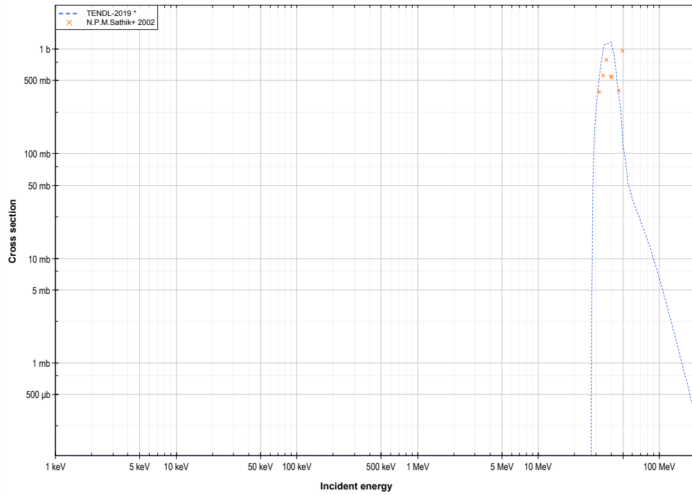
TI203 ( \alpha,3n ) or Bi204 production log-log
