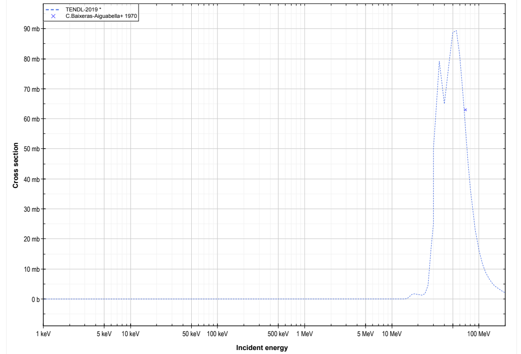
N14 ( \alpha, ^3\text{He} ) or N15 production lin-log
