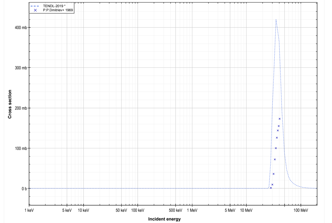
V51 ( \alpha,3n ) or Mn52 production lin-log
