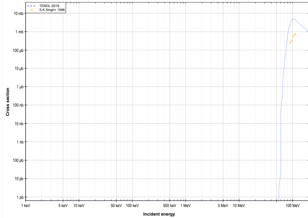
V51 ( \alpha,6n+p ) or Cr48 production log-log
