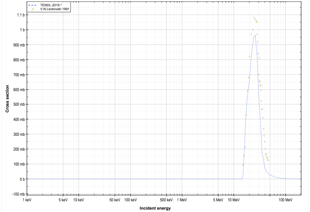
Se77 ( \alpha, 2n ) or Kr79 production lin-log
