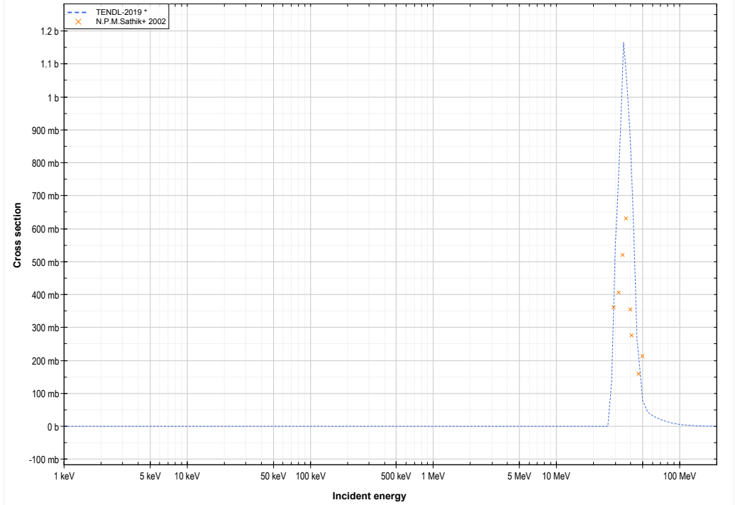
TI205 ( \alpha,3n ) or Bi206 production lin-log
