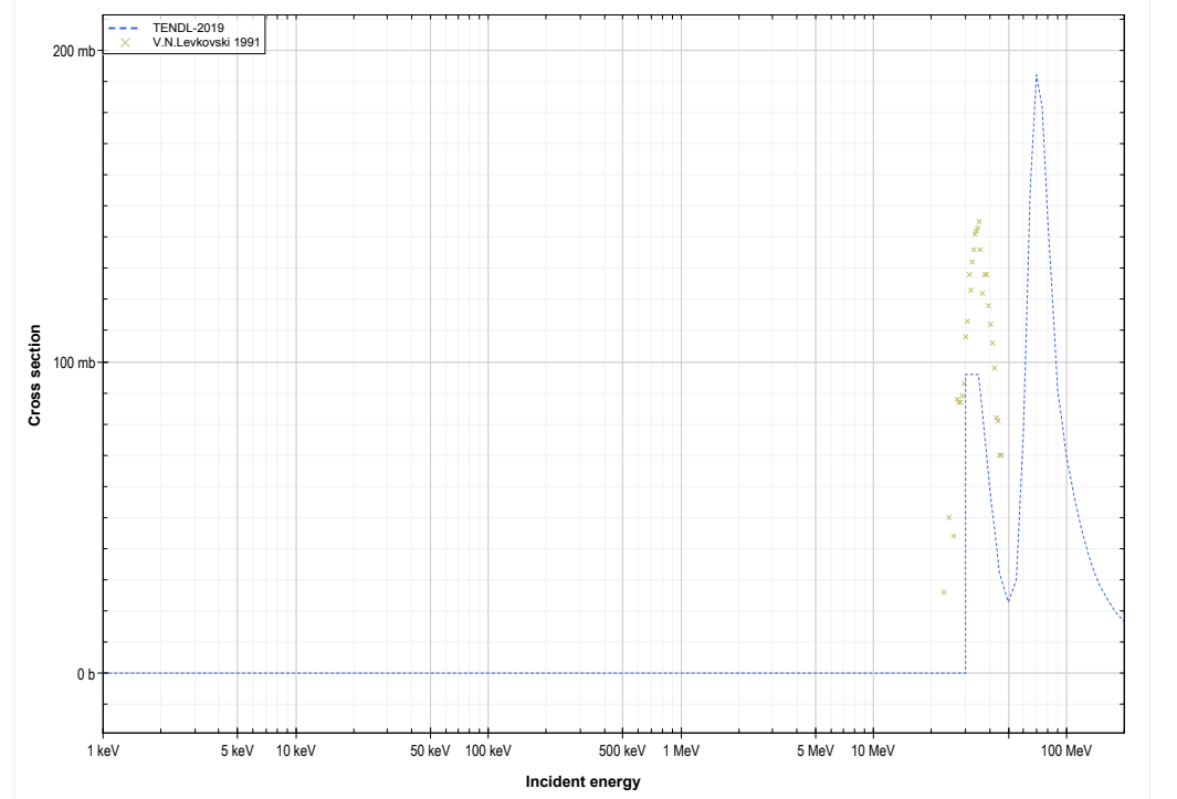
Zn64 ( \alpha, 2n+^3\text{He} ) or Zn63 production lin-log
