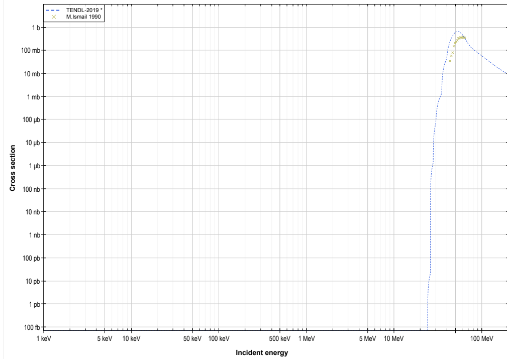
Ga69 ( \alpha, n+t ) or Ge69 production log-log
