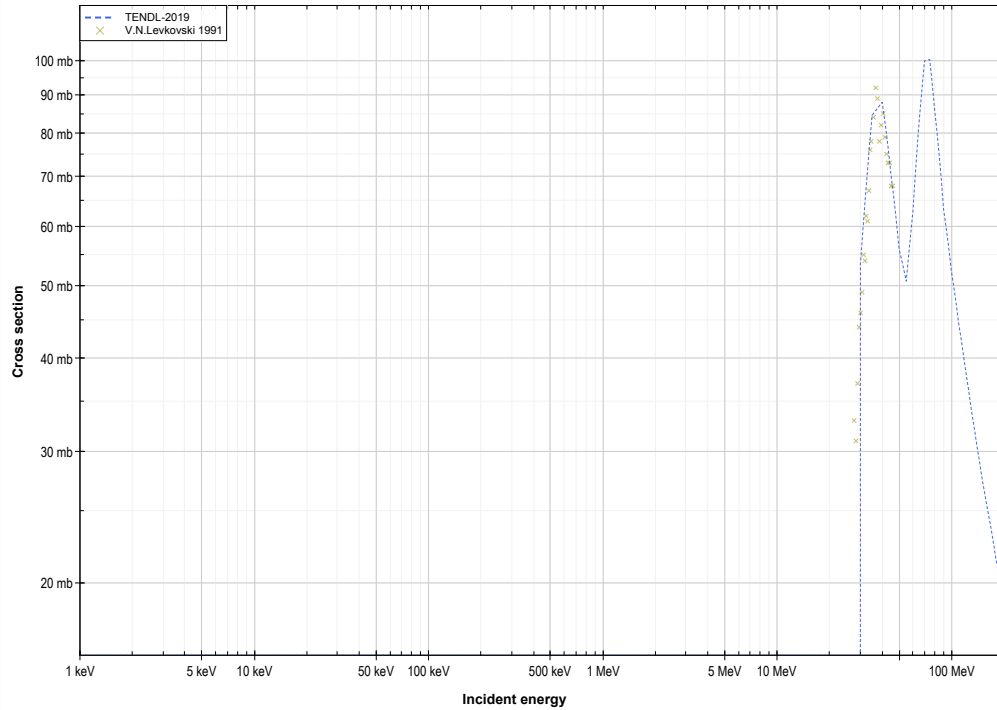
Y89 ( \alpha, n+p+t ) or Y88 production log-log
