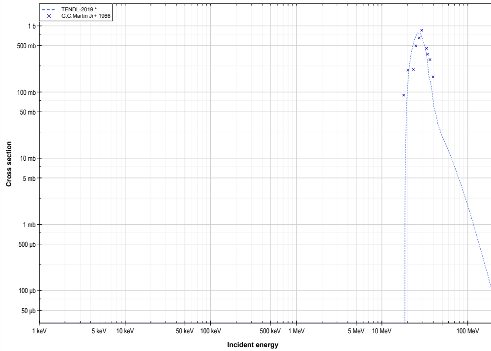
Er164 ( \alpha,2n ) or Yb166 production log-log
