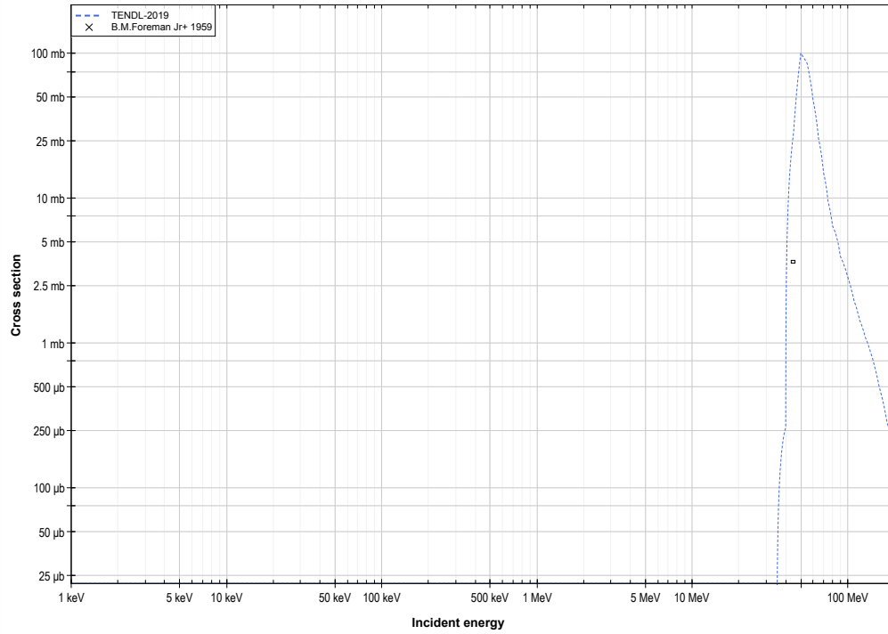
Th232 ( \alpha,5n ) or U231 production log-log
