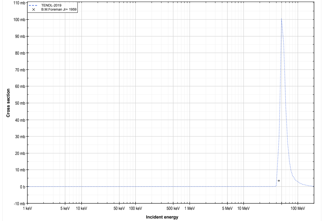
Th232 ( \alpha,5n ) or U231 production lin-log
