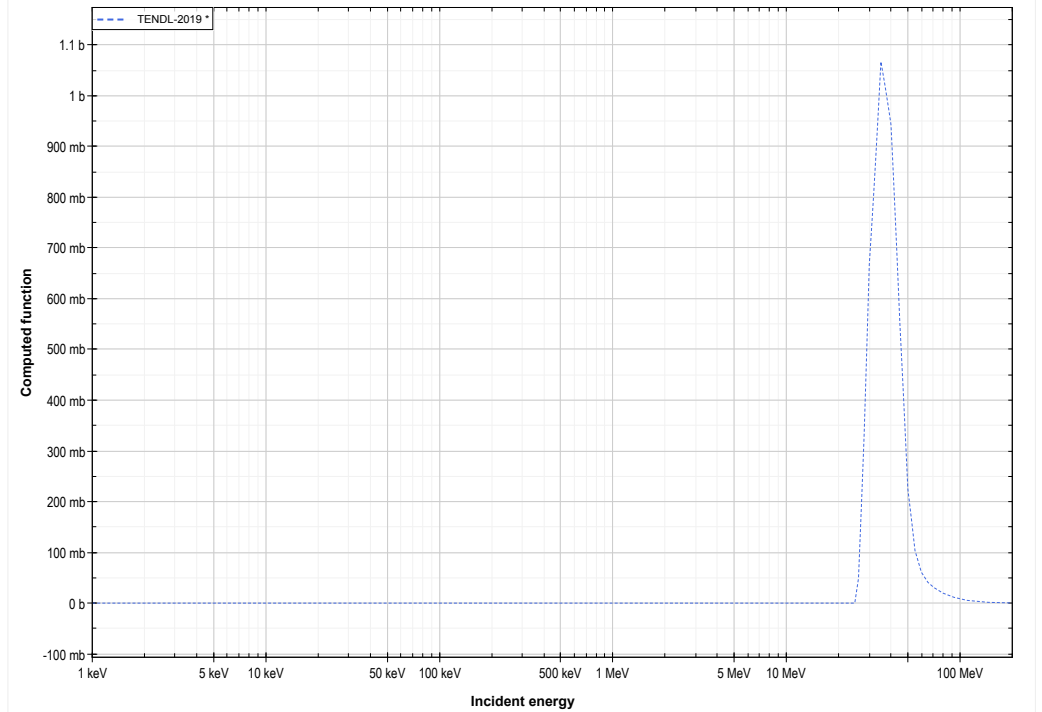
Br81 ( \alpha,3n ) or Rb82 production lin-log
