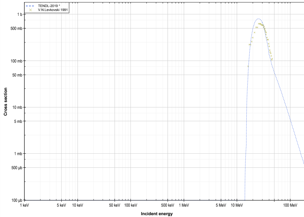
Ti46 ( \alpha,n+p ) or V48 production log-log
