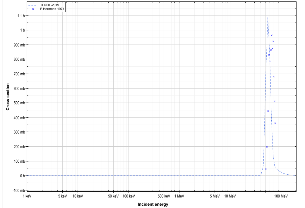
Ta181 ( \alpha,5n ) or Re180 production lin-log
