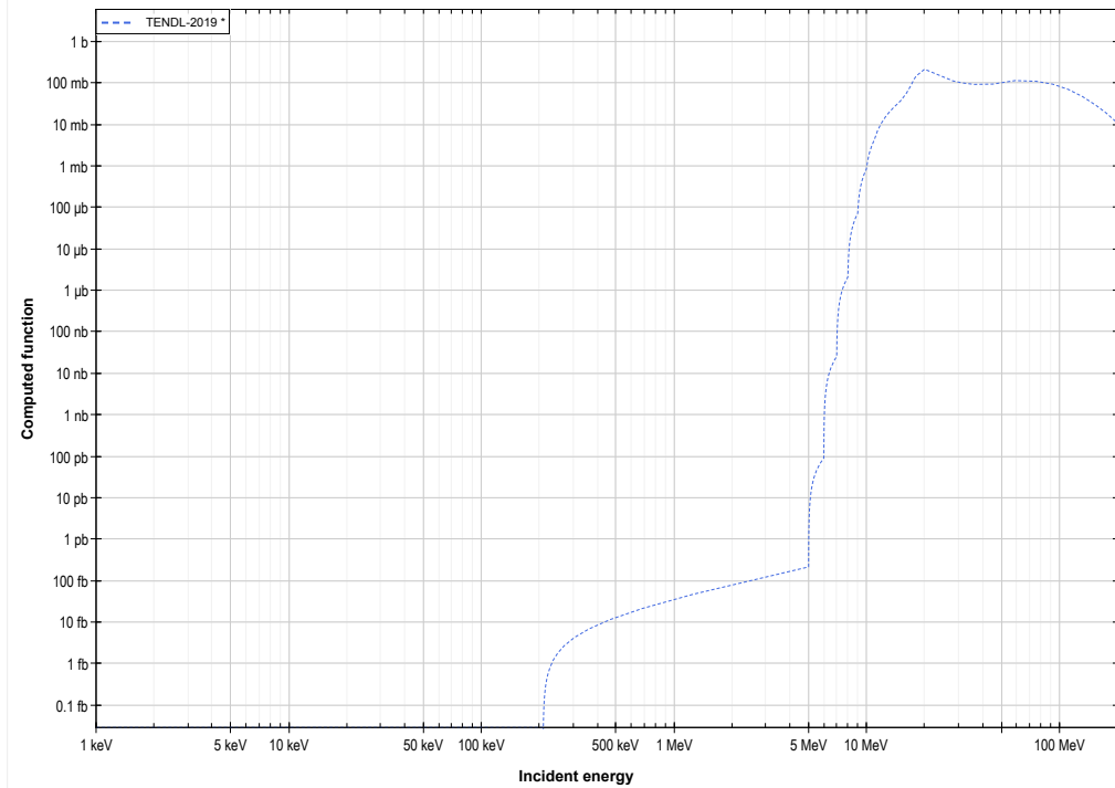
As75 ( \alpha,\alpha ) or As75 production log-log
