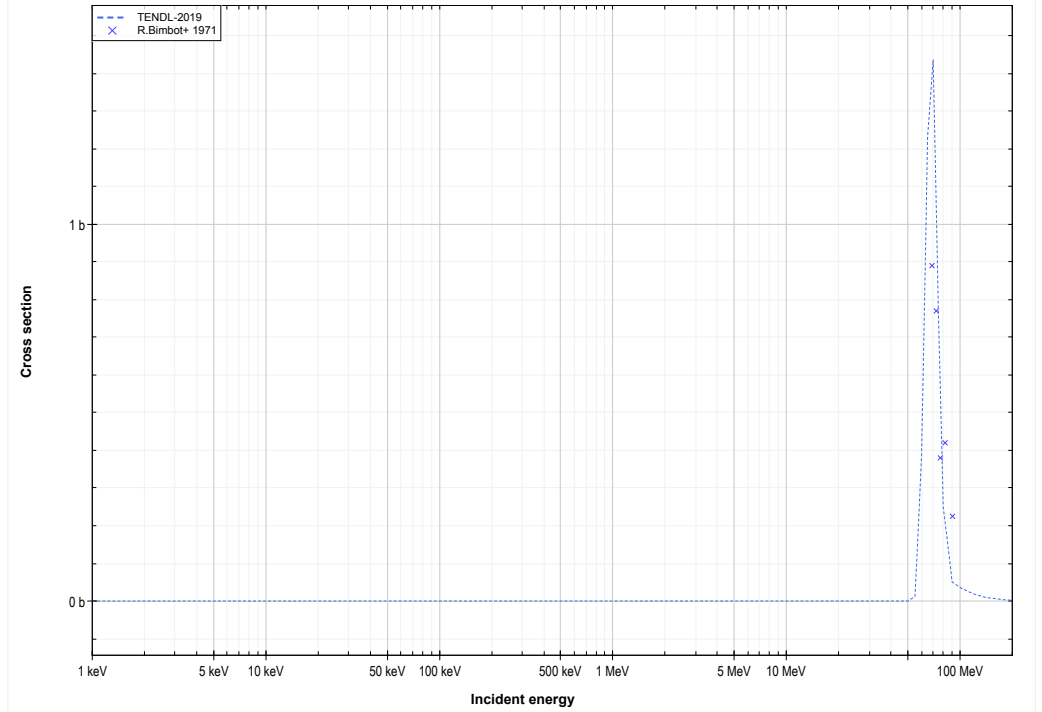
Pb208 ( \alpha, 6n ) or Po206 production lin-log
