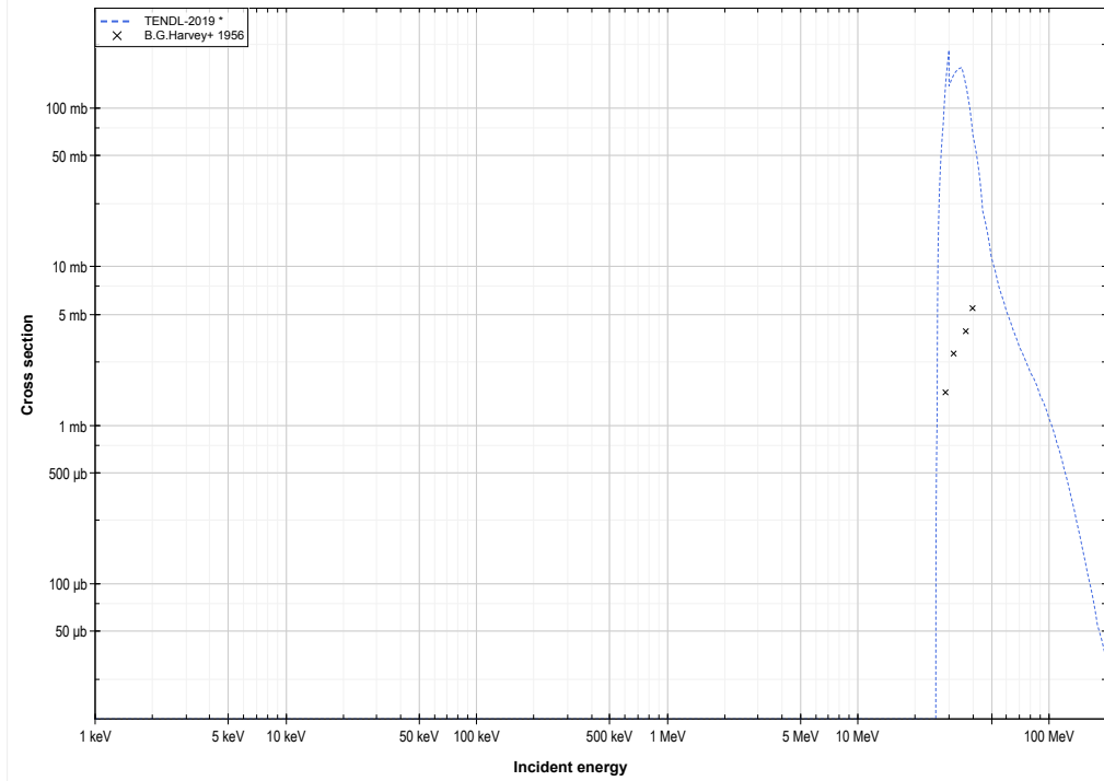
Bk249 ( \alpha,3n ) or Es250 production log-log
