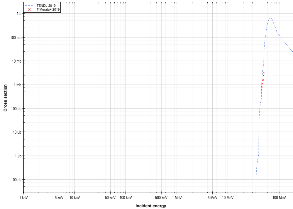
Y89 ( \alpha,2n+t ) or Zr88 production log-log
