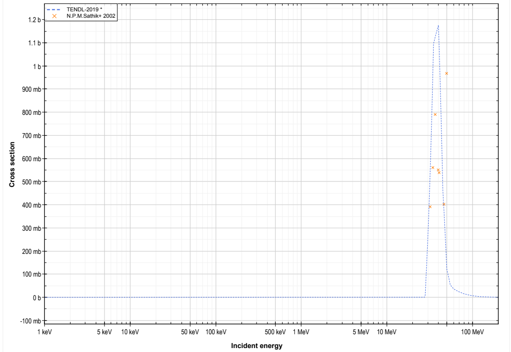
TI203 ( \alpha,3n ) or Bi204 production lin-log
