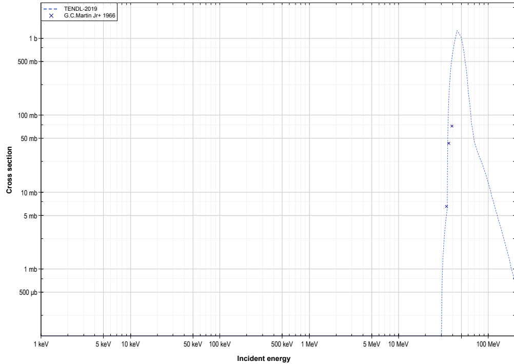
Er166 ( \alpha, 4n ) or Yb166 production log-log
