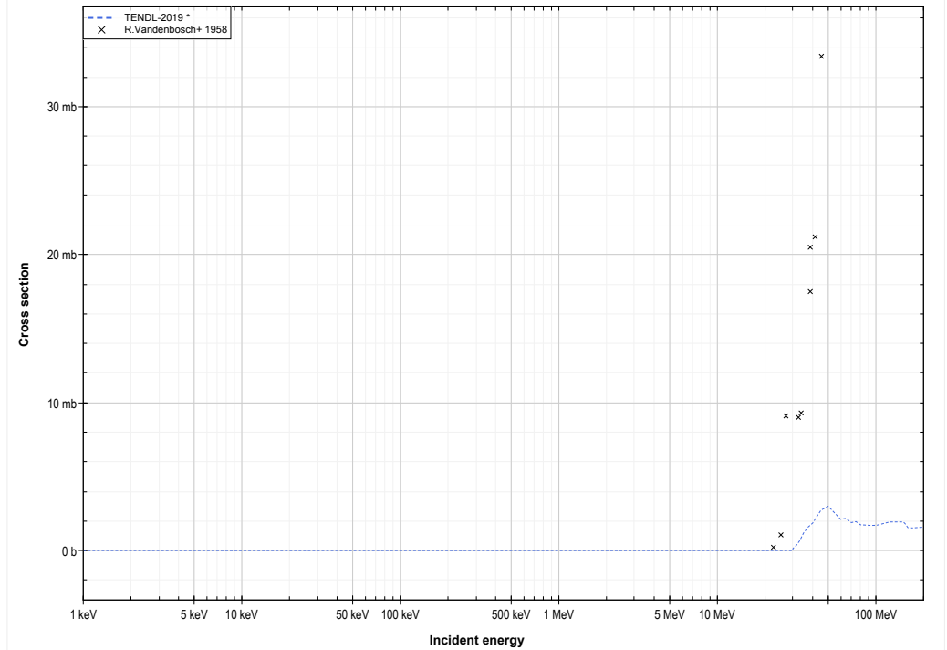
U238 ( \alpha,2n+p ) or Np239 production lin-log
