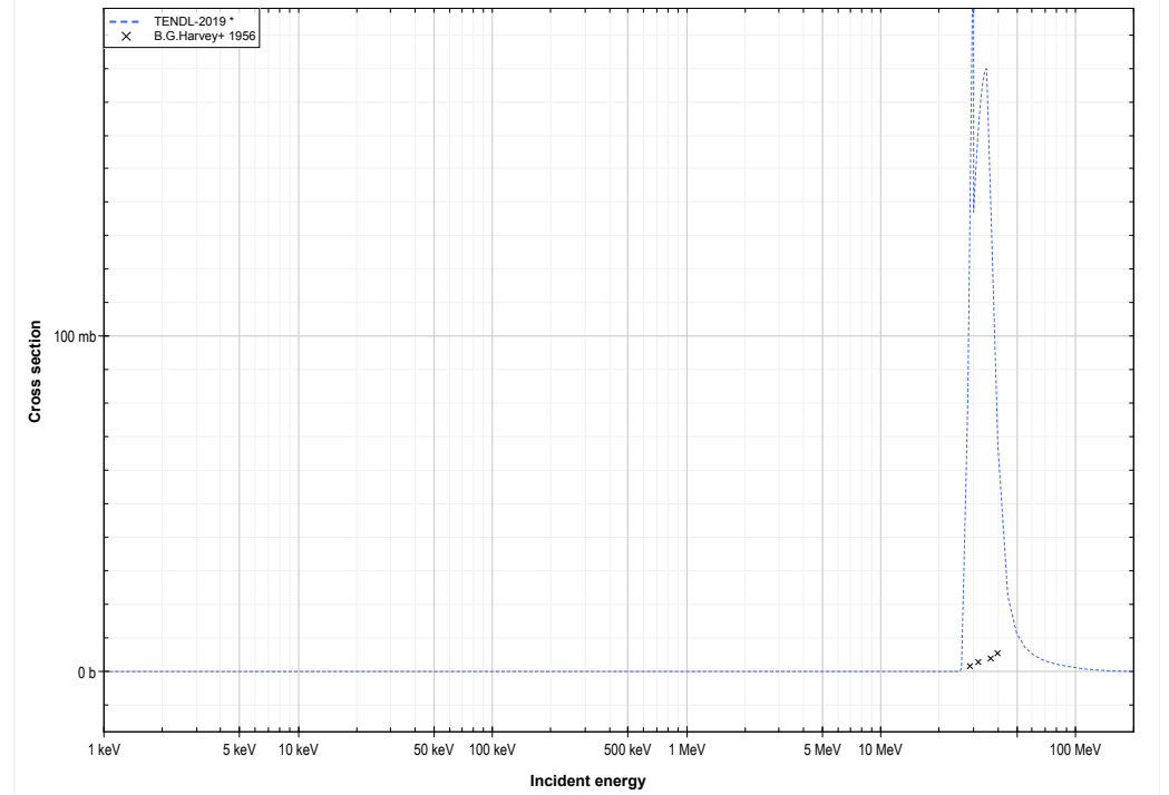
Bk249 ( \alpha,3n ) or Es250 production lin-log
