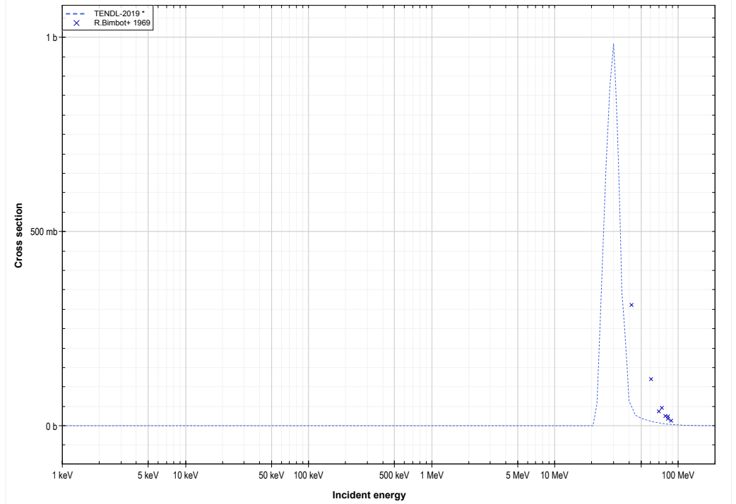
Pb206 ( \alpha,2n ) or Po208 production lin-log
