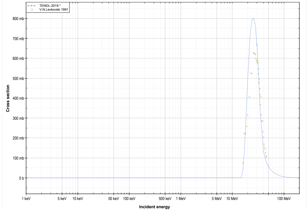
Ti46 ( \alpha,n+p ) or V48 production lin-log
