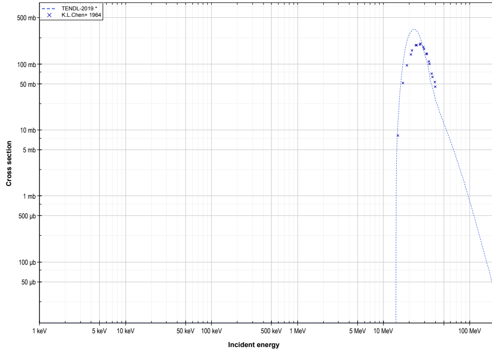
Sc45 ( \alpha, 2n ) or V47 production log-log
