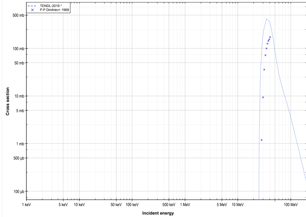
V51 ( \alpha,3n ) or Mn52 production log-log
