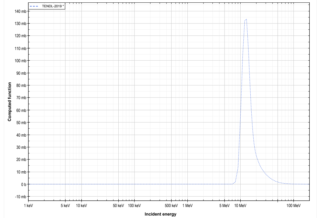
Se82 ( \alpha, n ) or Kr85 production lin-log
