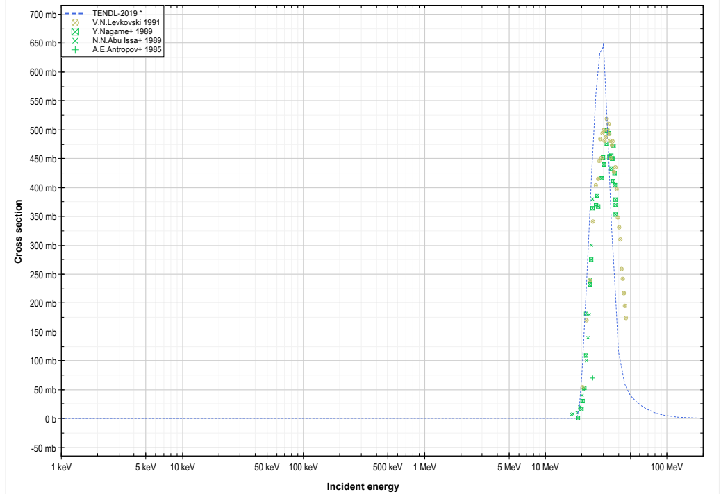
Zn66 ( \alpha, n+p ) or Ga68 production lin-log
