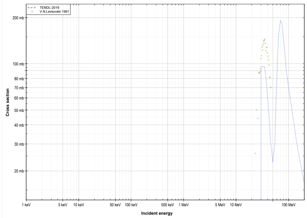
Zn64 ( \alpha, 2n+^3\text{He} ) or Zn63 production log-log
