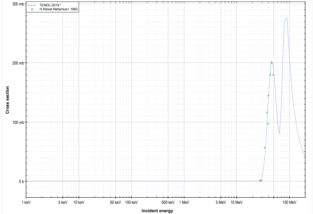
V51 ( \alpha,2n+\alpha ) or V49 production lin-log
