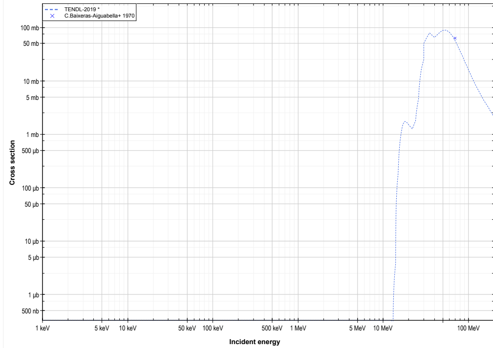
N14 ( \alpha, ^3\text{He} ) or N15 production log-log
