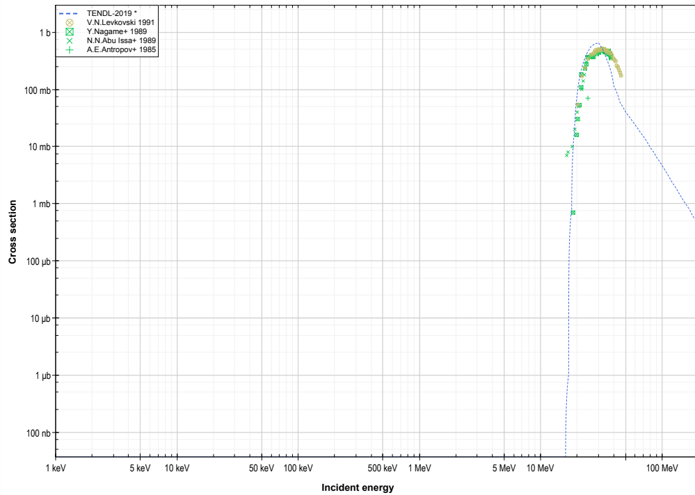
Zn66 ( \alpha, n+p ) or Ga68 production log-log
