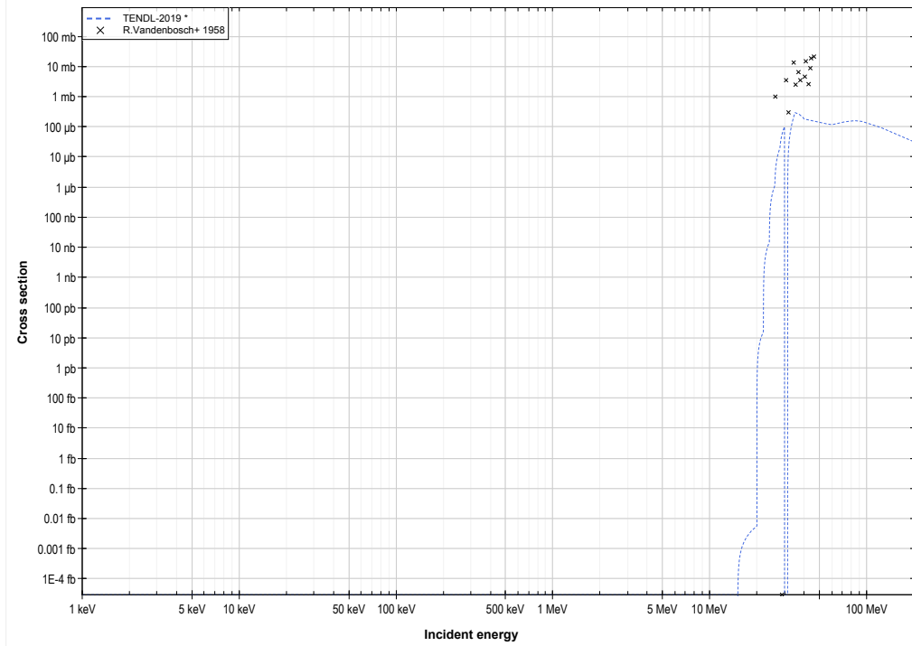
U233 ( \alpha,d ) or Np235 production log-log
