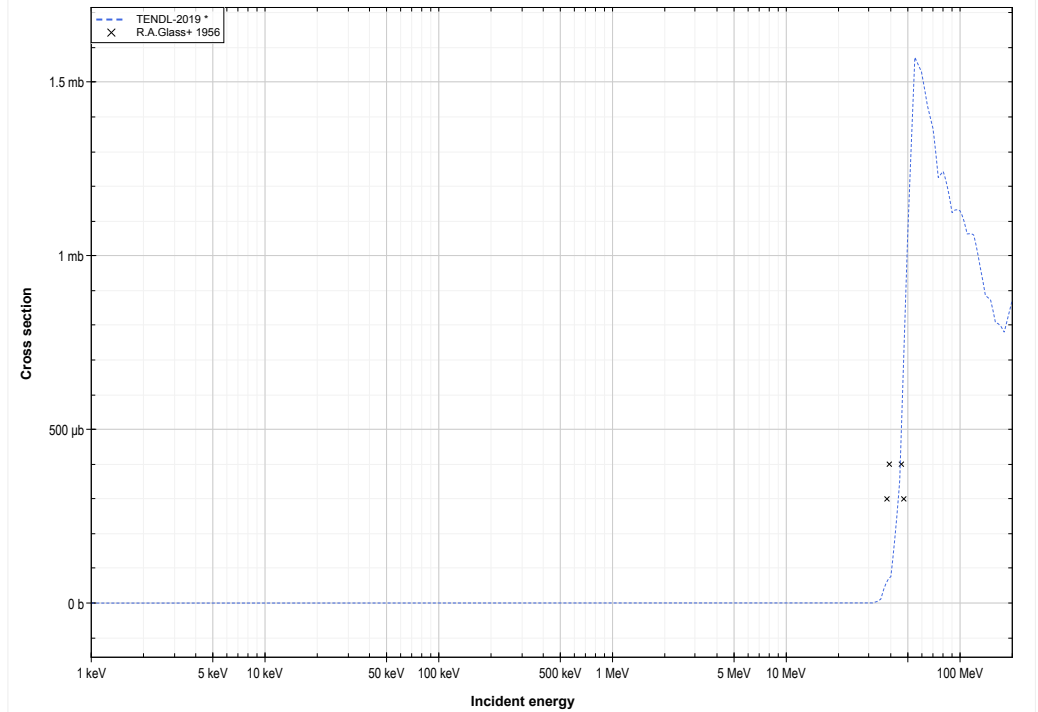
Pu239 ( \alpha, n+t ) or Am239 production lin-log
