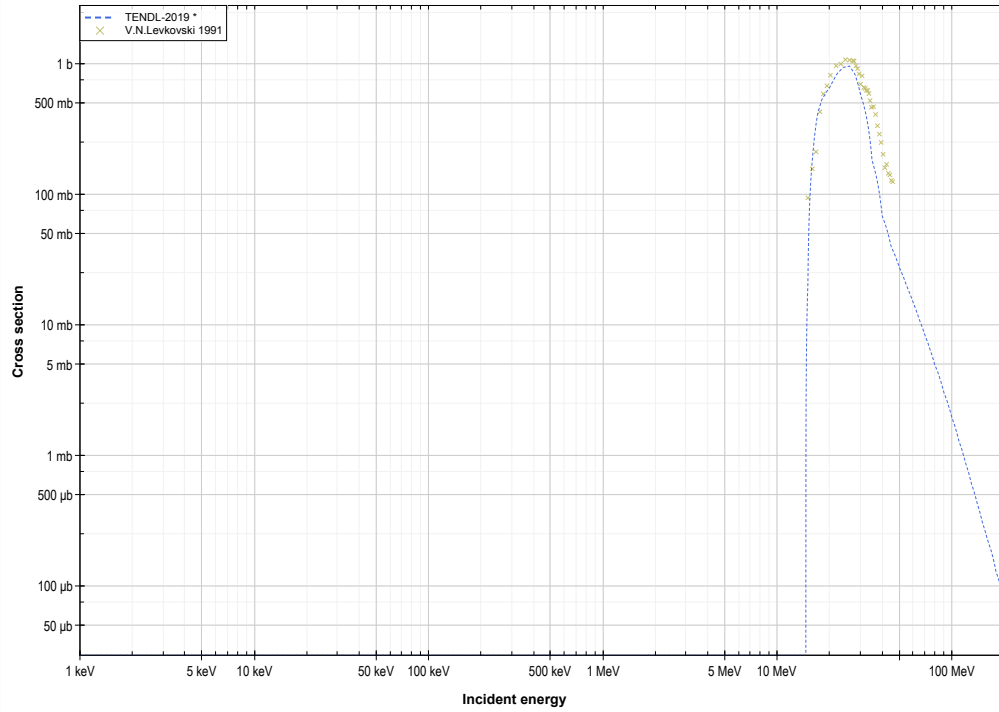
Se77 ( \alpha, 2n ) or Kr79 production log-log
