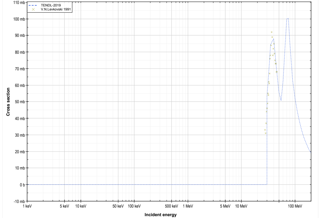
Y89 ( \alpha, n+p+t ) or Y88 production lin-log
