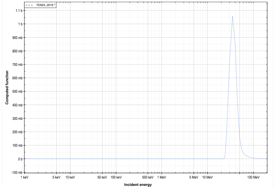
Zn70 ( \alpha, 3n ) or Ge71 production lin-log
