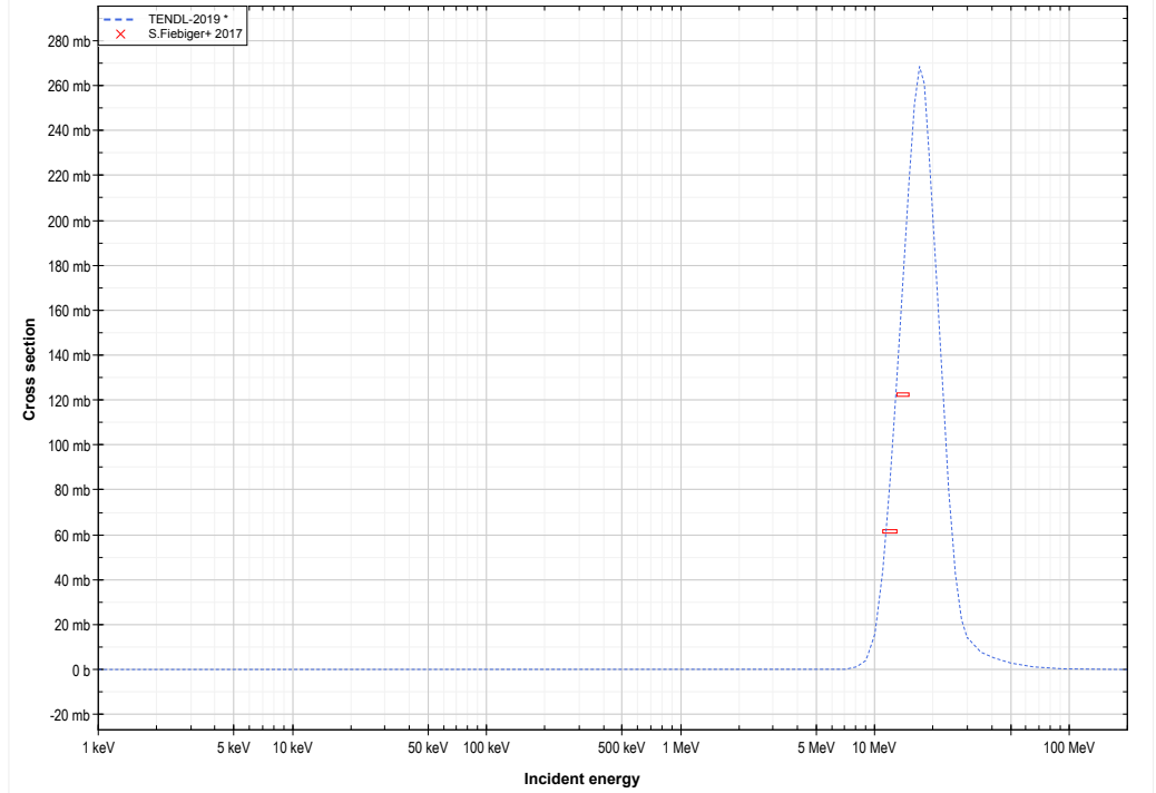
Se74 ( \alpha, p ) or Br77 production lin-log
