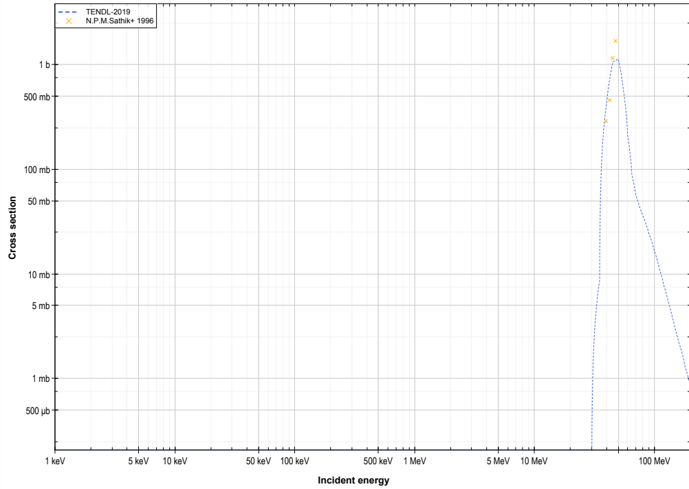
Cs133 ( \alpha,4n ) or La133 production log-log
