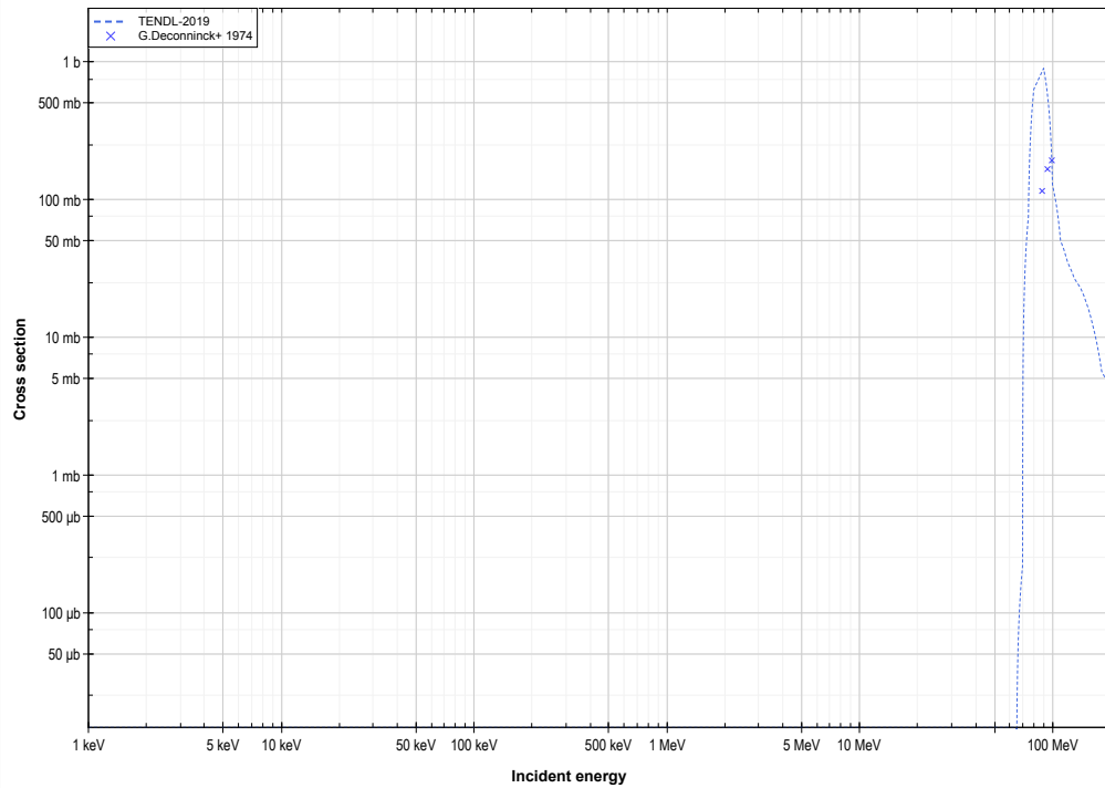
Bi209 ( \alpha,8n ) or At205 production log-log
