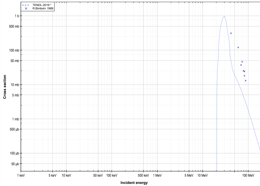
Pb206 ( \alpha,2n ) or Po208 production log-log
