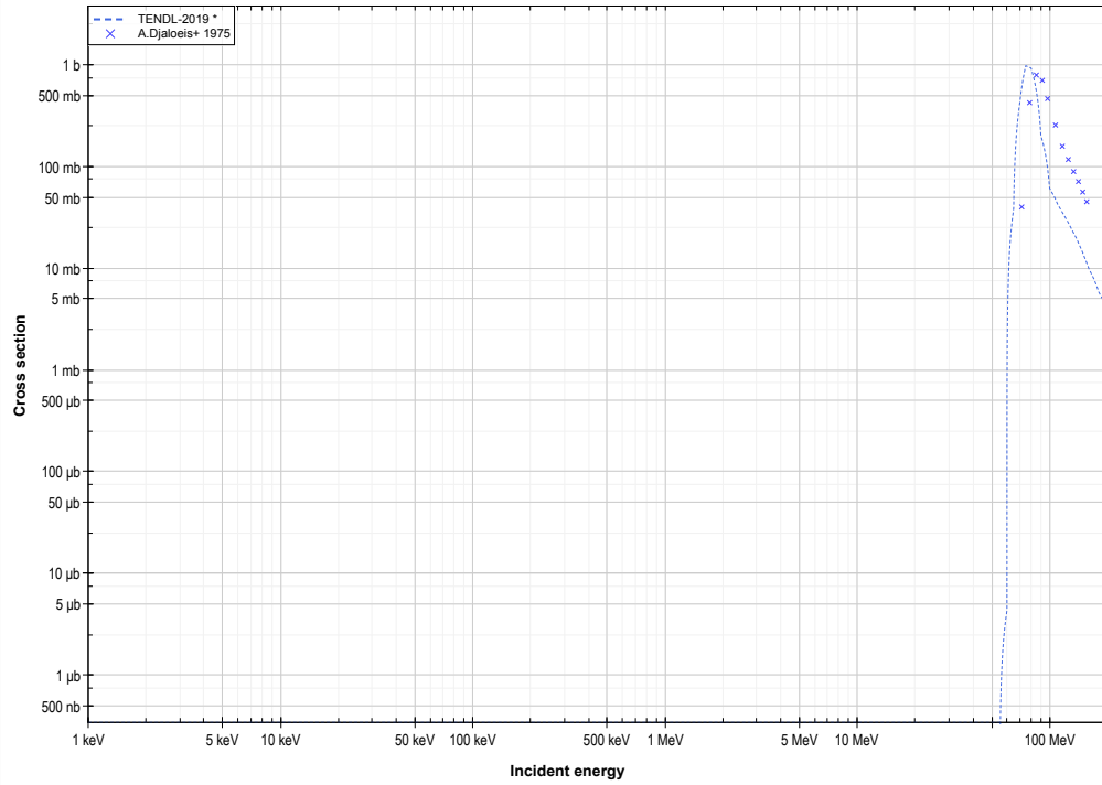
Au197 ( \alpha,7n ) or Tl194 production log-log
