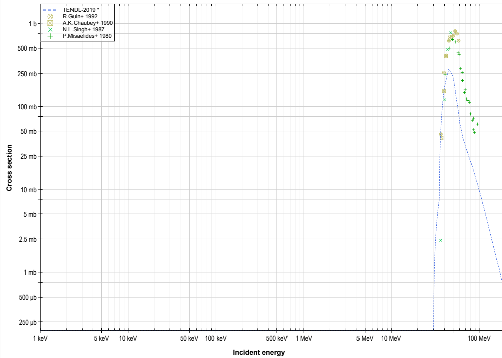
Ag109 ( \alpha,4n ) or In109 production log-log
