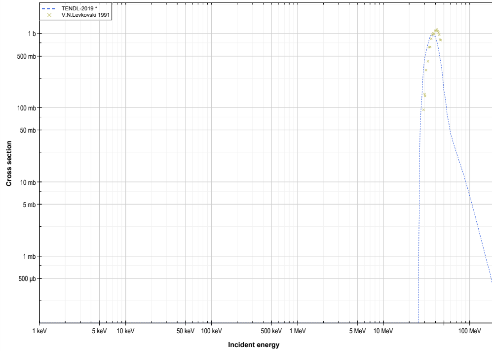
Mo96 ( \alpha,3n ) or Ru97 production log-log
