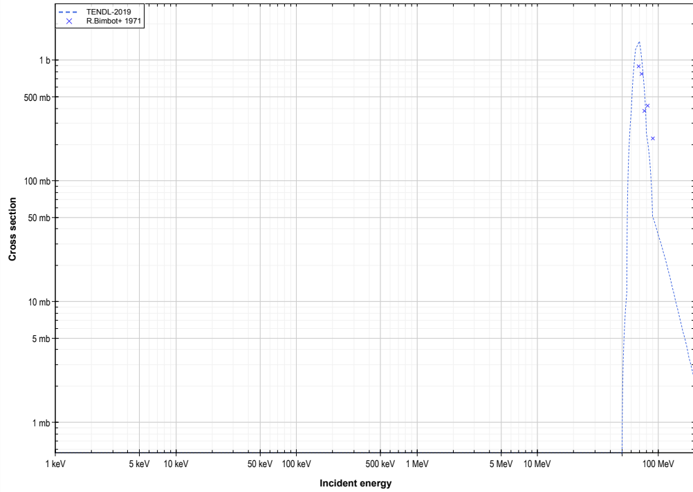
Pb208 ( \alpha, 6n ) or Po206 production log-log
