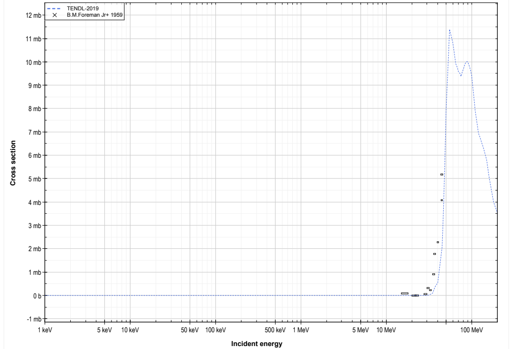
Th232 ( \alpha,3n+p ) or Pa232 production lin-log
