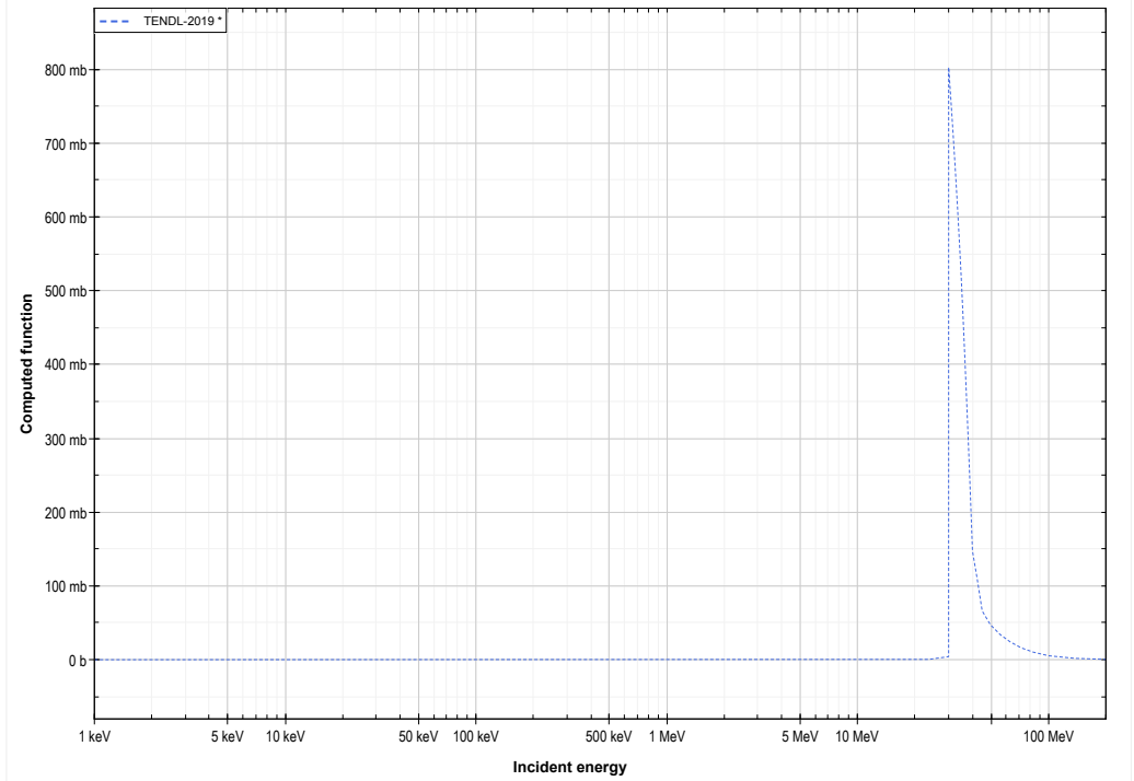
Mo92 ( \alpha,d ) or Tc94 production lin-log
