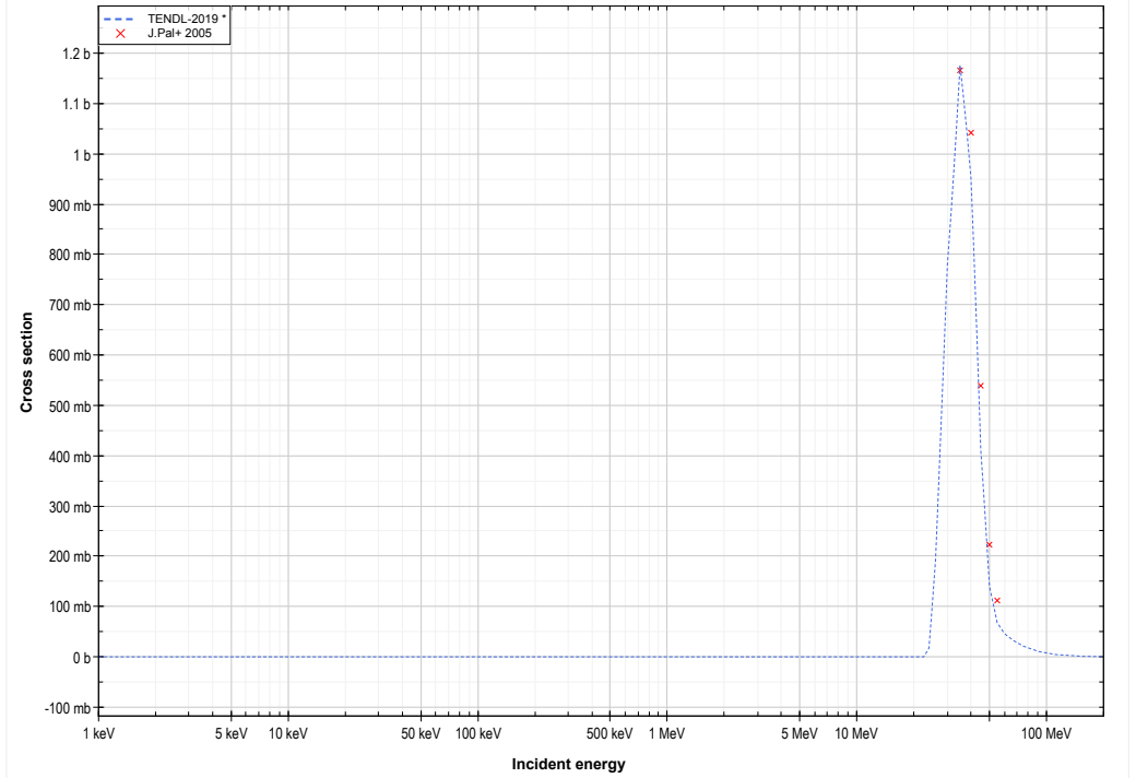
Cd114 ( \alpha,3n ) or Sn115 production lin-log
