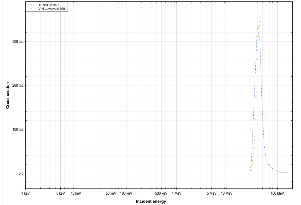
Se76 ( \alpha,3n ) or Kr77 production lin-log
