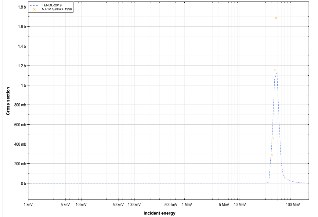
Cs133 ( \alpha,4n ) or La133 production lin-log
