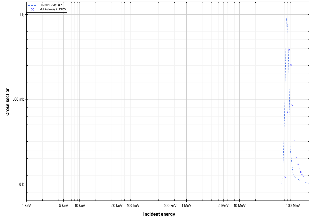
Au197 ( \alpha,7n ) or Tl194 production lin-log
