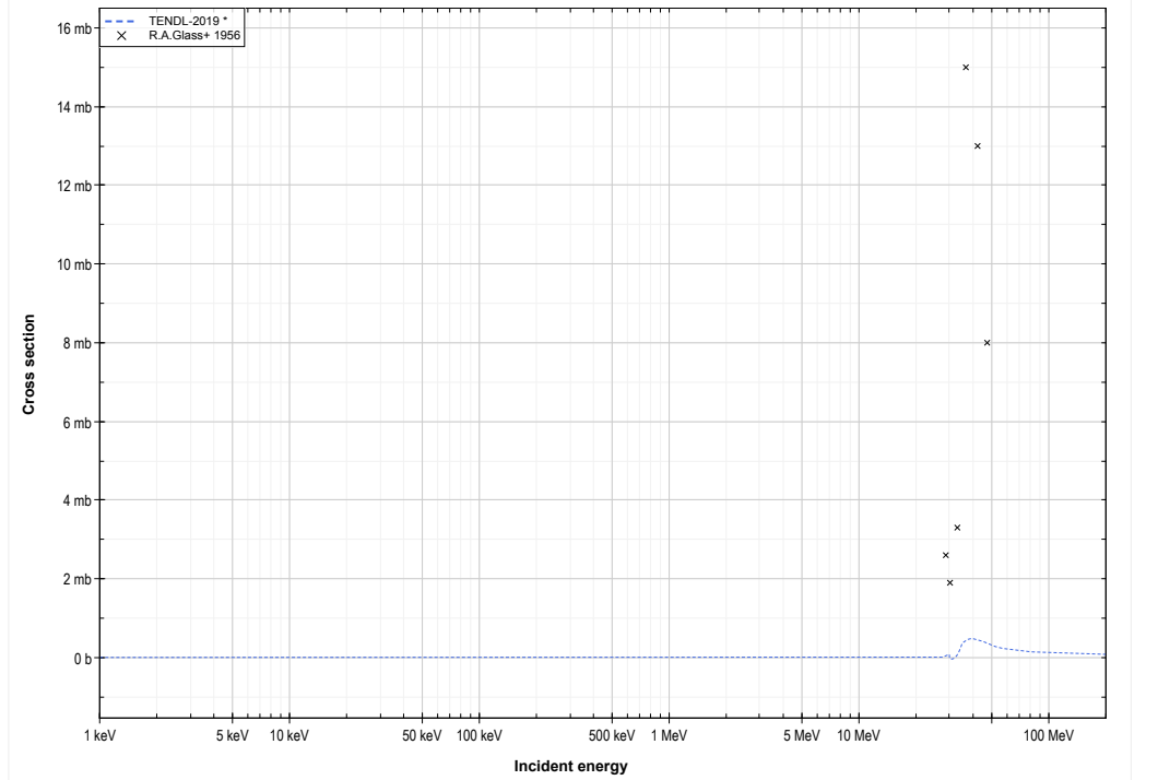
Pu238 ( \alpha,d ) or Am240 production lin-log
