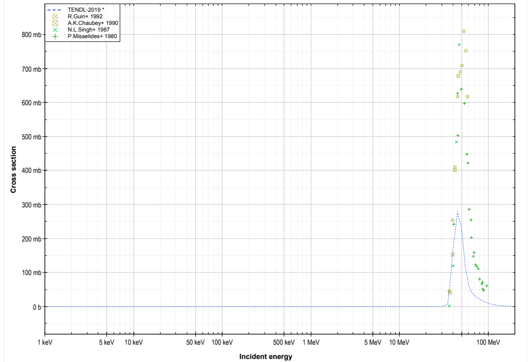
Ag109 ( \alpha,4n ) or In109 production lin-log
