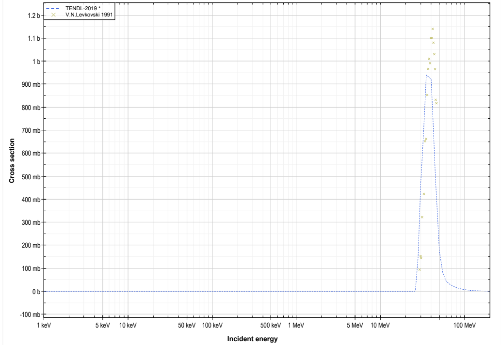
Mo96 ( \alpha,3n ) or Ru97 production lin-log
