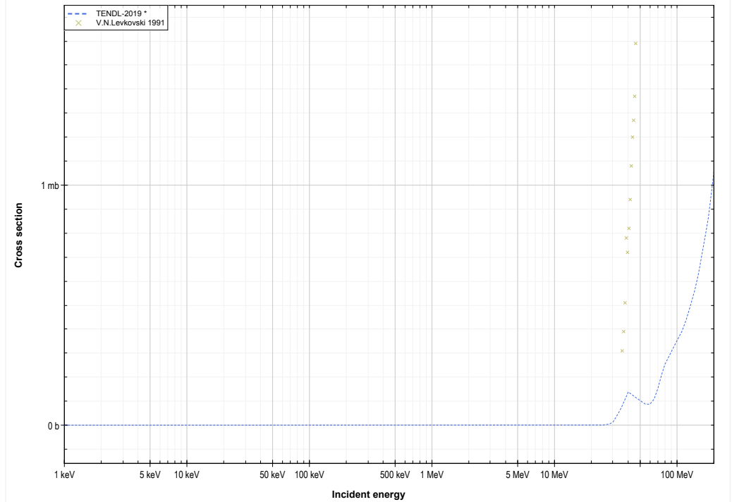
Ge74 ( \alpha, p + \alpha ) or Ga73 production lin-log
