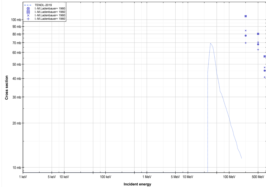
I127 ( \alpha,2n+^3\text{He} ) or I126 production log-log
