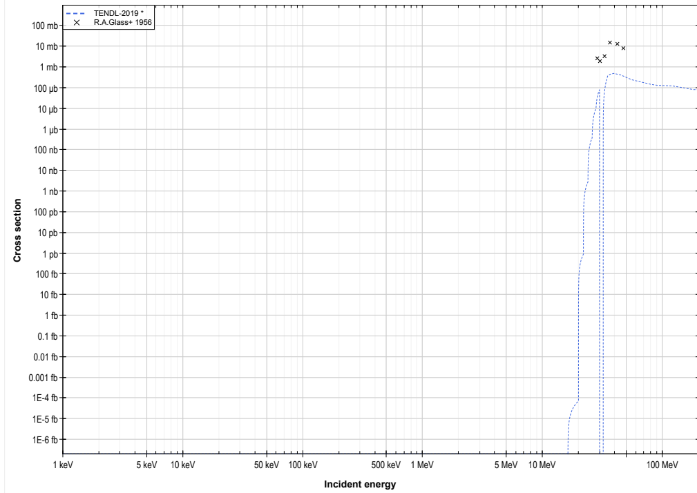
Pu238 ( \alpha,d ) or Am240 production log-log
