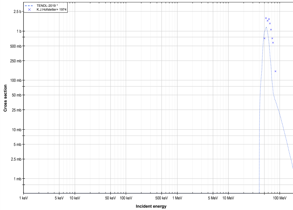
Re187 ( \alpha,5n ) or Ir186 production log-log
