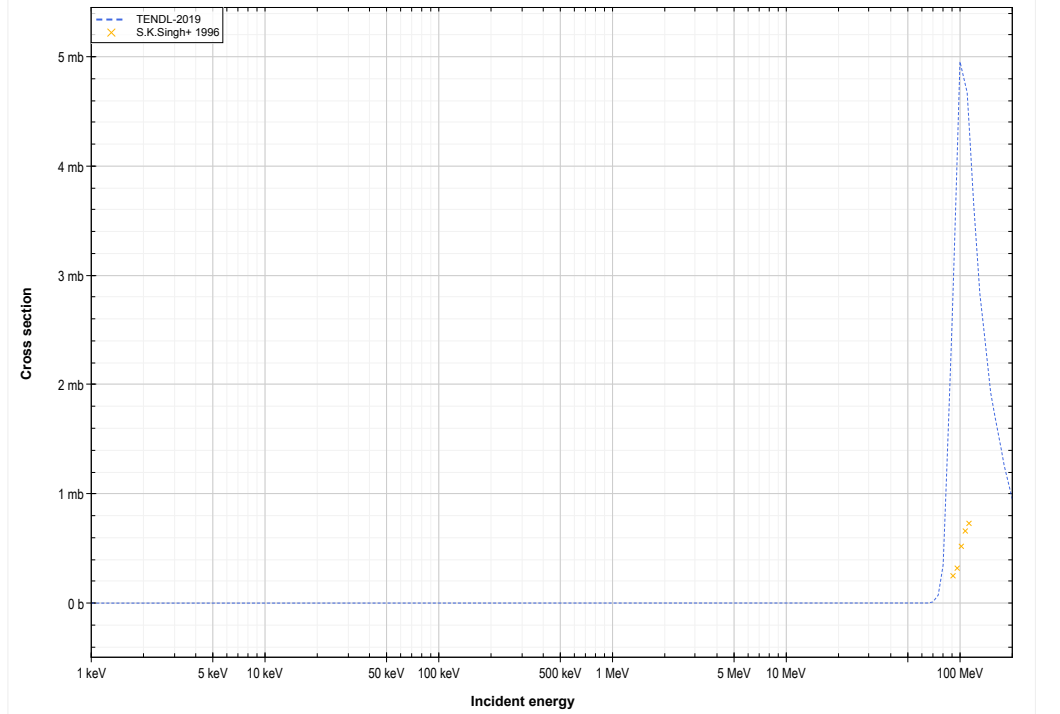
V51 ( \alpha,6n+p ) or Cr48 production lin-log
