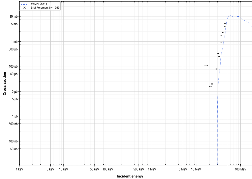
Th232 ( \alpha,3n+p ) or Pa232 production log-log
