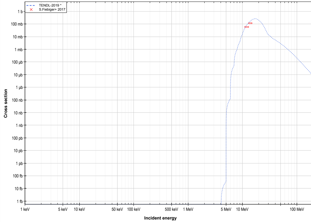
Se74 ( \alpha, p ) or Br77 production log-log
