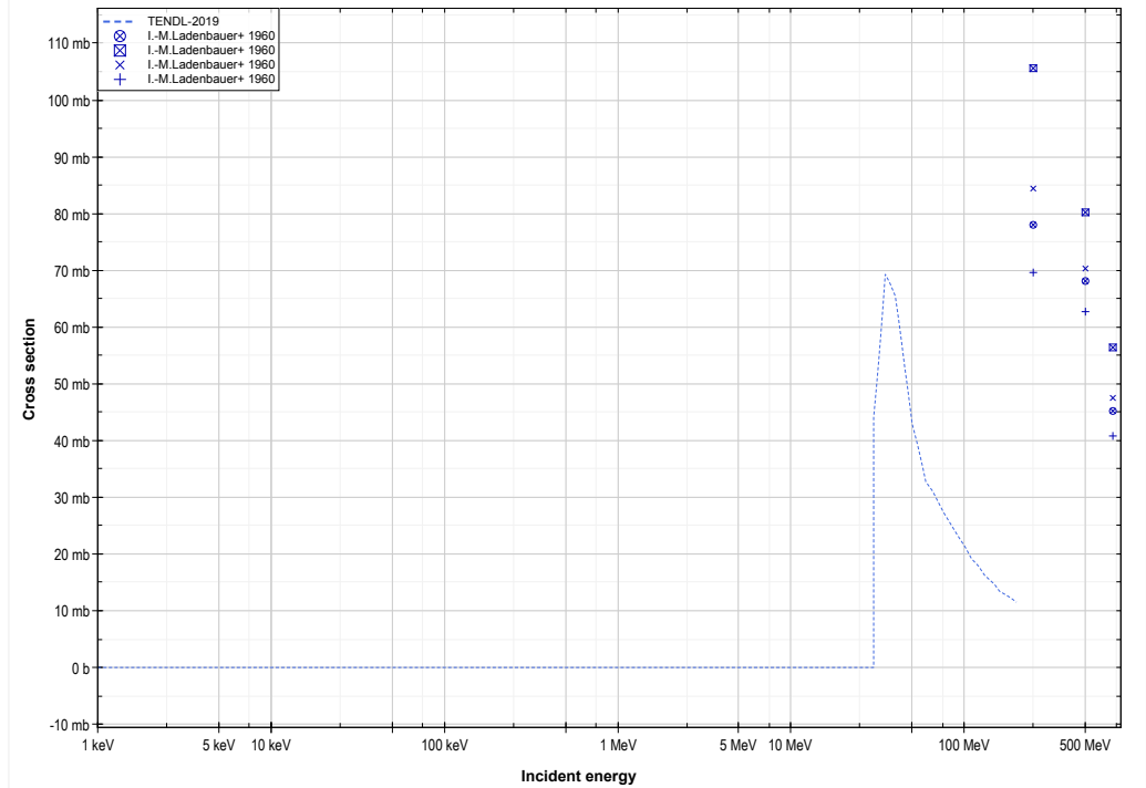
I127 ( \alpha,2n+^3\text{He} ) or I126 production lin-log
