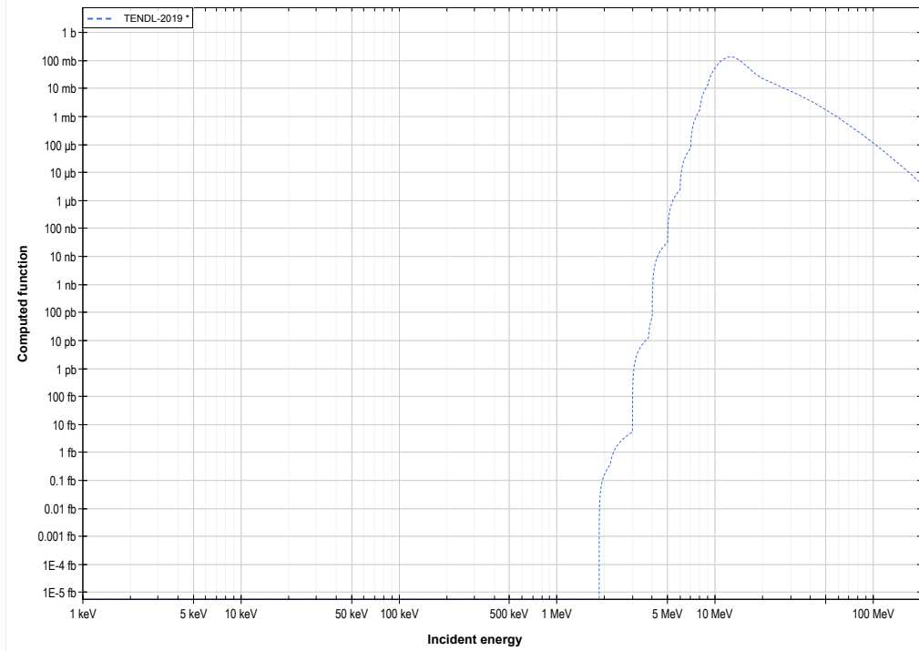
Se82 ( \alpha, n ) or Kr85 production log-log
