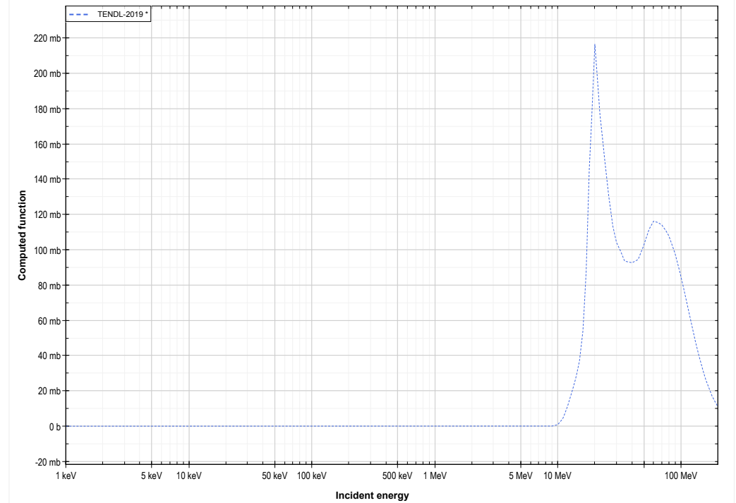
As75 ( \alpha,\alpha ) or As75 production lin-log
