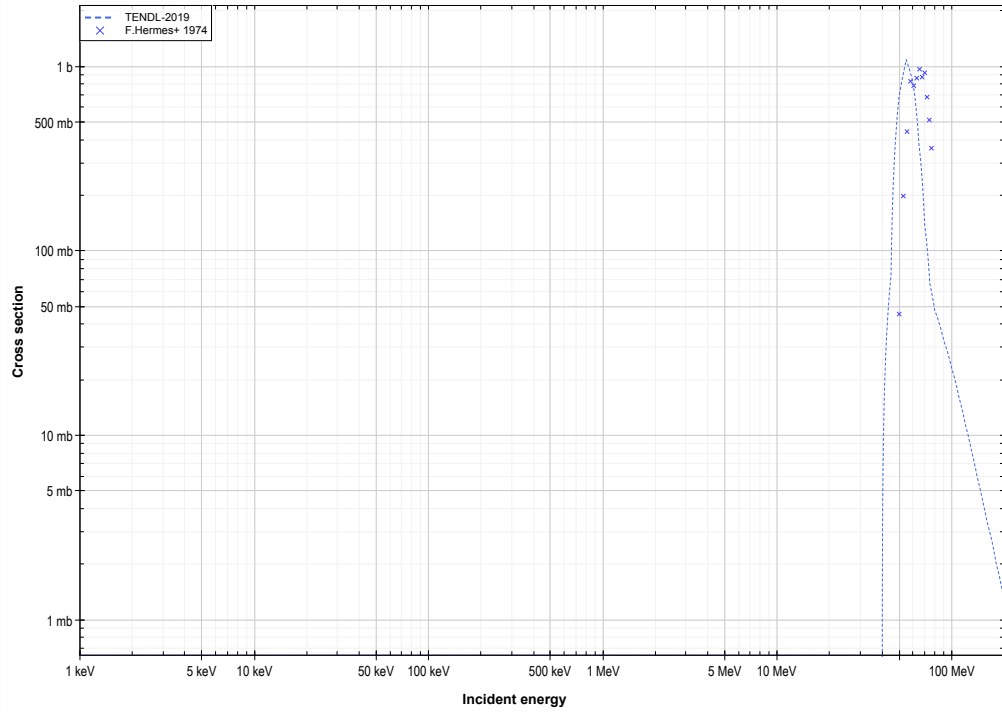
Ta181 ( \alpha,5n ) or Re180 production log-log
