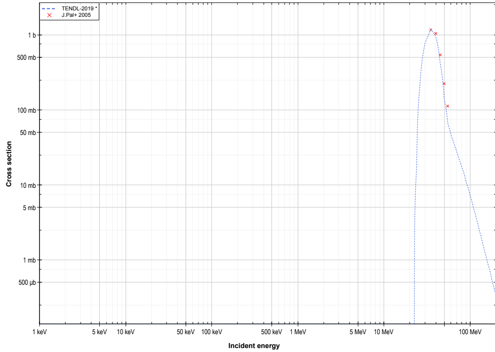
Cd114 ( \alpha,3n ) or Sn115 production log-log
