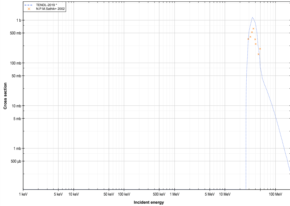
TI205 ( \alpha,3n ) or Bi206 production log-log
