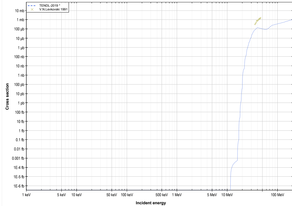
Ge74 ( \alpha, p + \alpha ) or Ga73 production log-log
