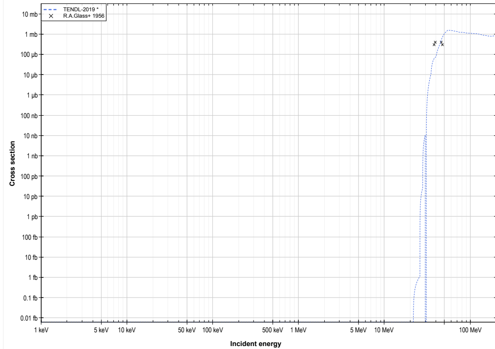
Pu239 ( \alpha, n+t ) or Am239 production log-log
