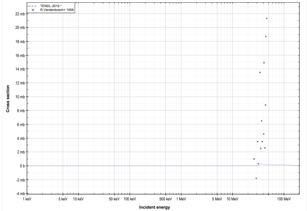
U233 ( \alpha,d ) or Np235 production lin-log
