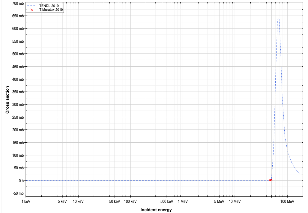
Y89 ( \alpha,2n+t ) or Zr88 production lin-log
