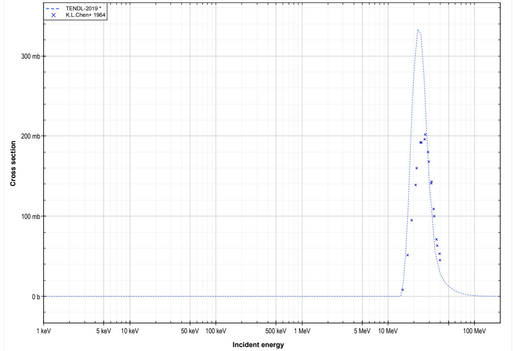
Sc45 ( \alpha, 2n ) or V47 production lin-log
