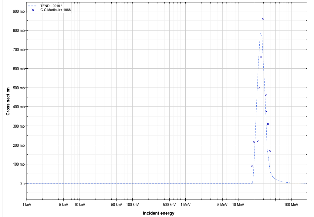
Er164 ( \alpha,2n ) or Yb166 production lin-log
