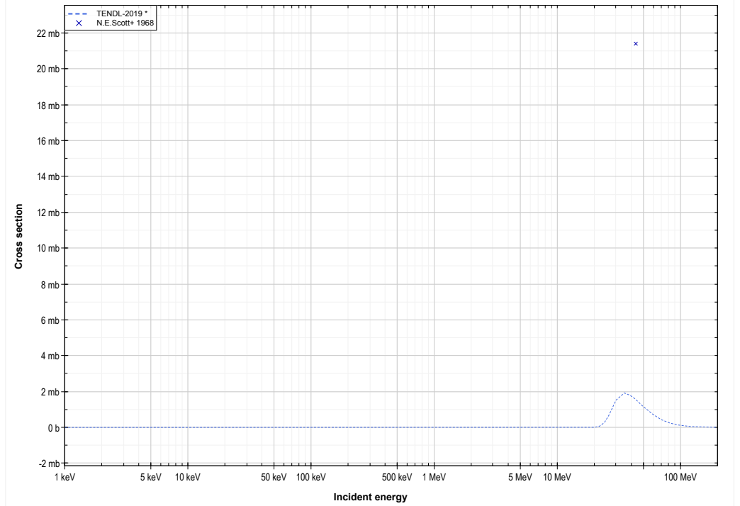
W186 ( \alpha, p ) or Re189 production lin-log
