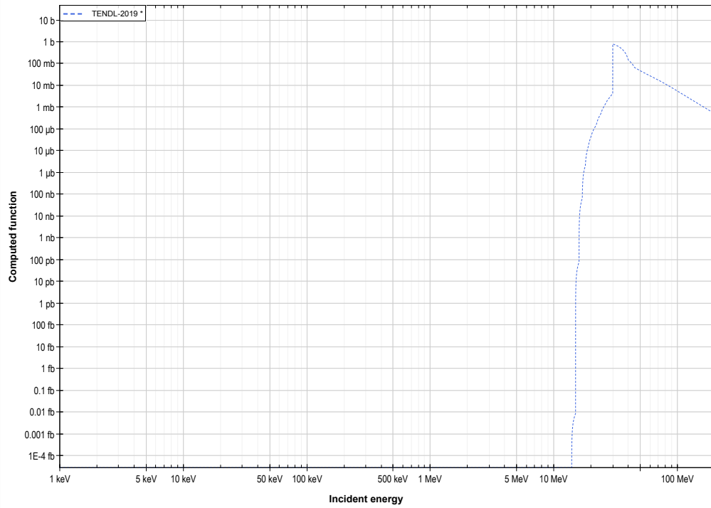
Mo92 ( \alpha,d ) or Tc94 production log-log
