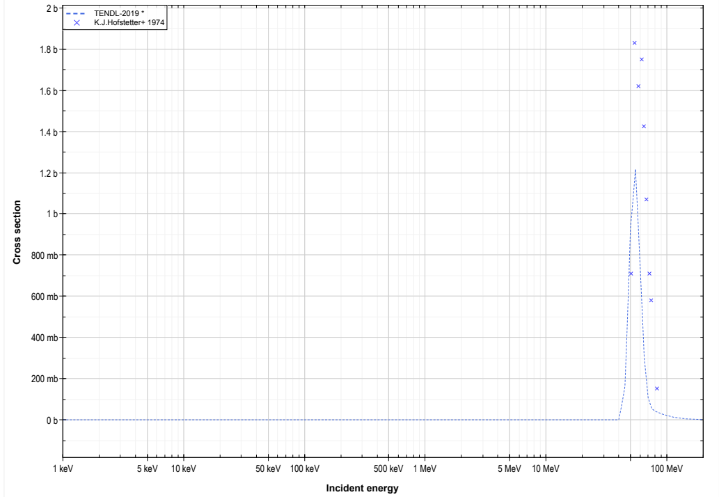
Re187 ( \alpha,5n ) or Ir186 production lin-log
