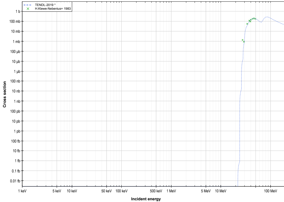
V51 ( \alpha,2n+\alpha ) or V49 production log-log
