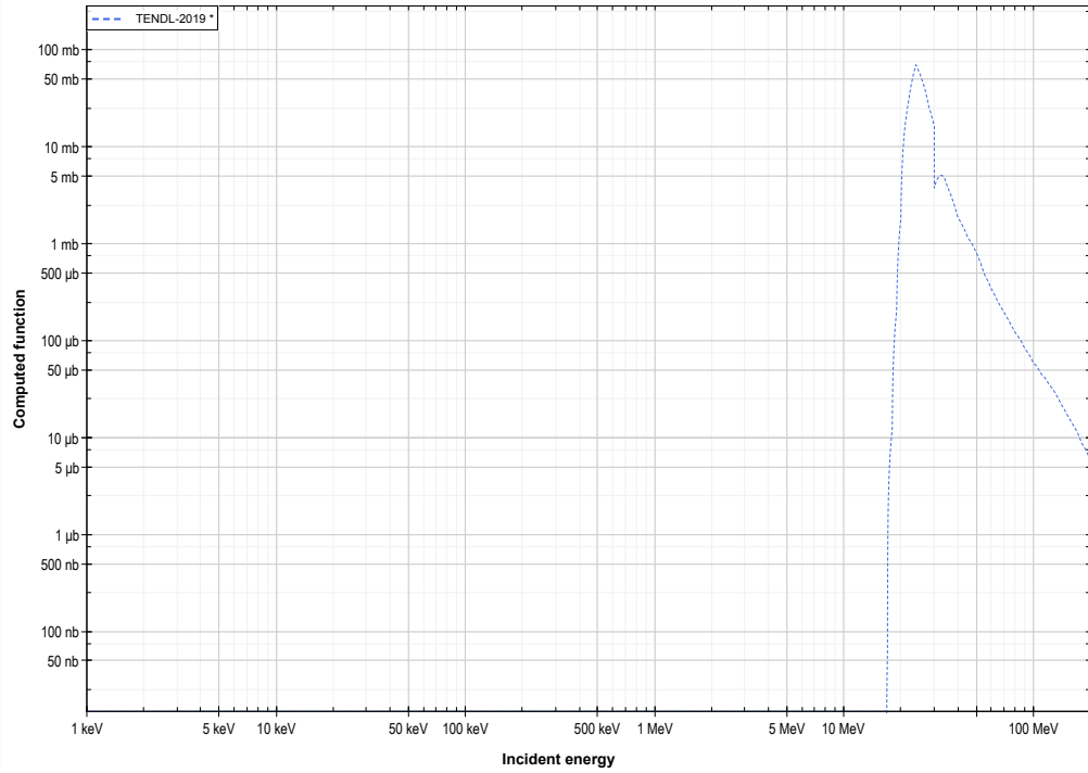
U238 ( \alpha,2n ) or Pu240 production log-log
