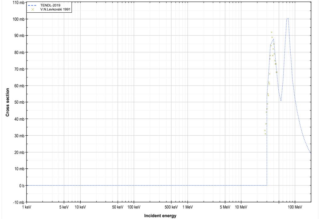
Y89 ( \alpha, 3n+2p ) or Y88 production lin-log
