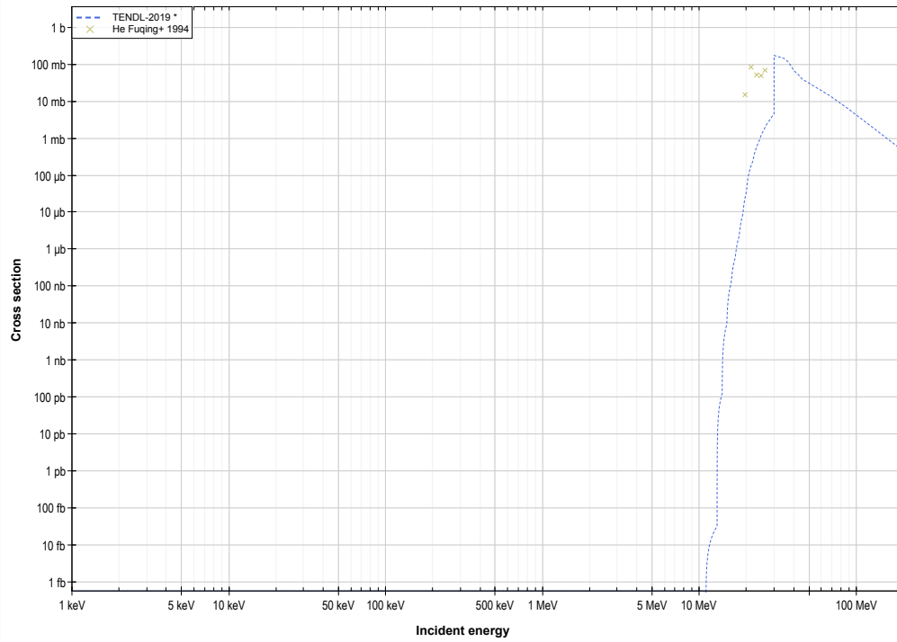
Ag107 ( \alpha,d ) or Cd109 production log-log
