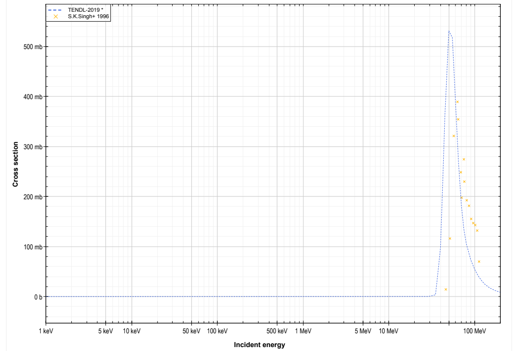
V51 ( \alpha, n+t ) or Cr51 production lin-log
