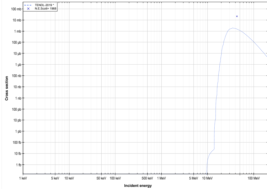
W186 ( \alpha, p ) or Re189 production log-log
