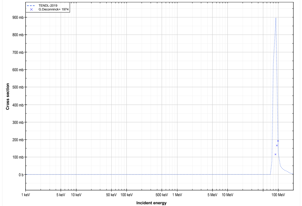
Bi209 ( \alpha,8n ) or At205 production lin-log
