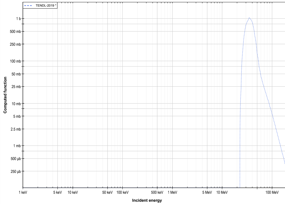
Zn70 ( \alpha, 3n ) or Ge71 production log-log
