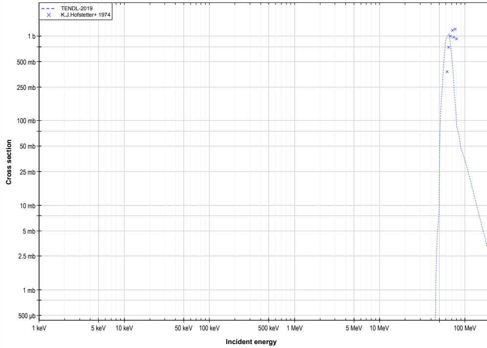
Re187 ( \alpha,6n ) or Ir185 production log-log
