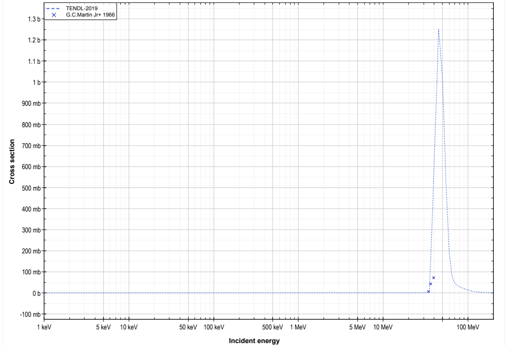
Er166 ( \alpha, 4n ) or Yb166 production lin-log
