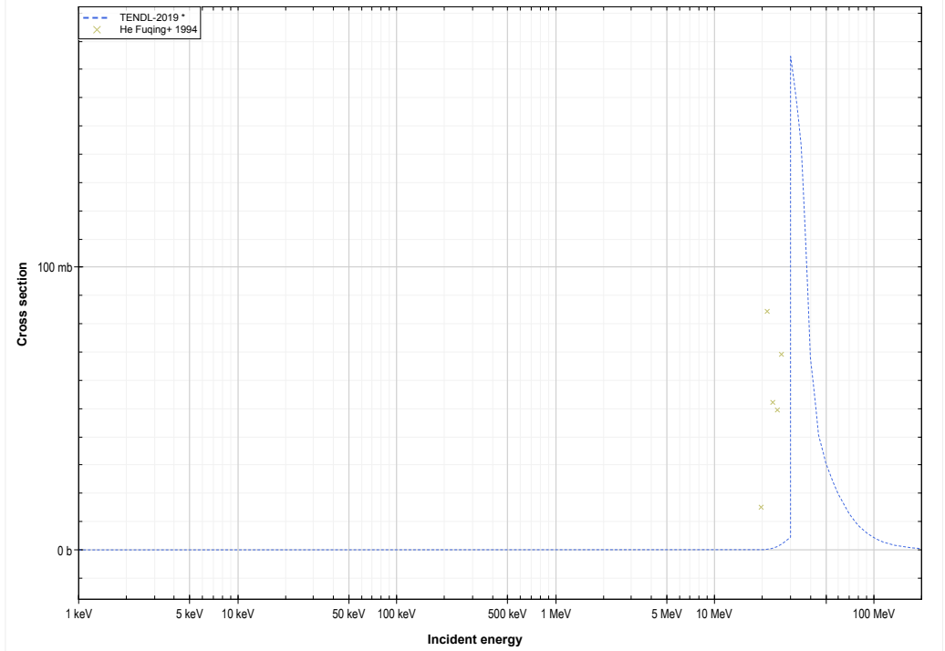
Ag107 ( \alpha,d ) or Cd109 production lin-log
