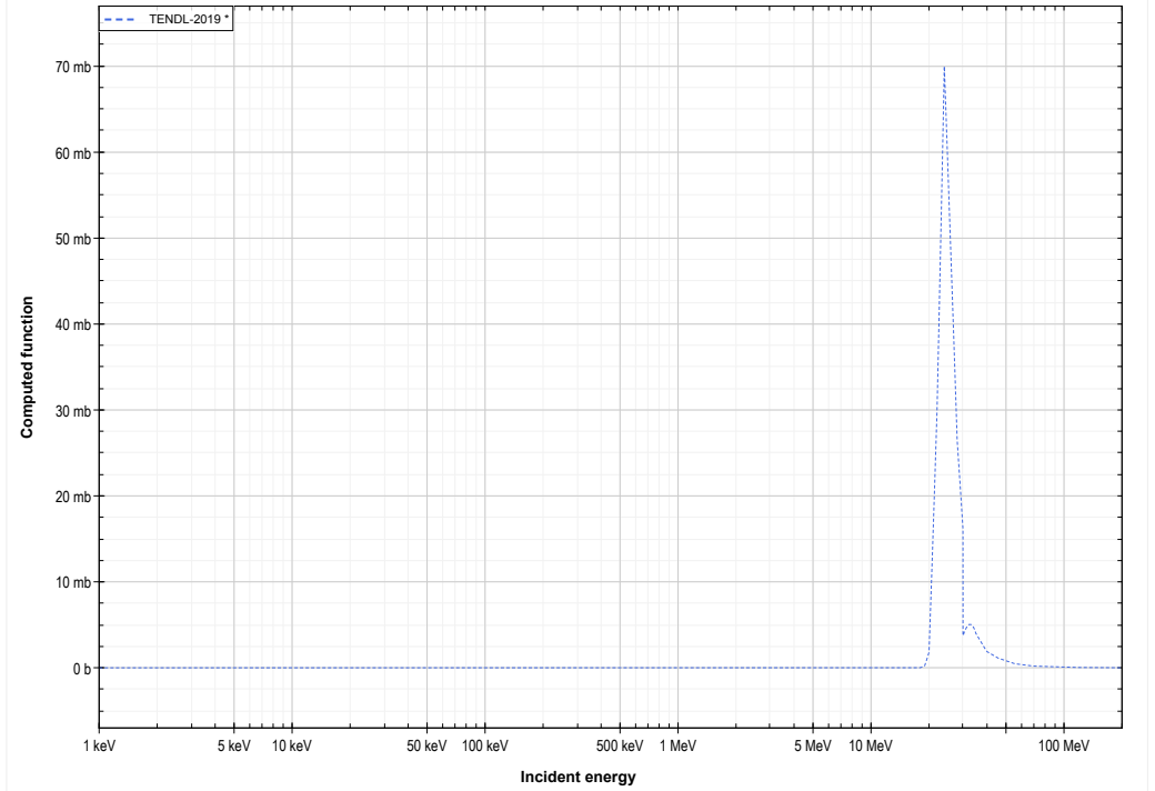
U238 ( \alpha,2n ) or Pu240 production lin-log
