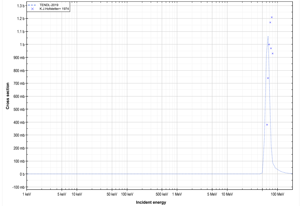
Re187 ( \alpha,6n ) or Ir185 production lin-log
