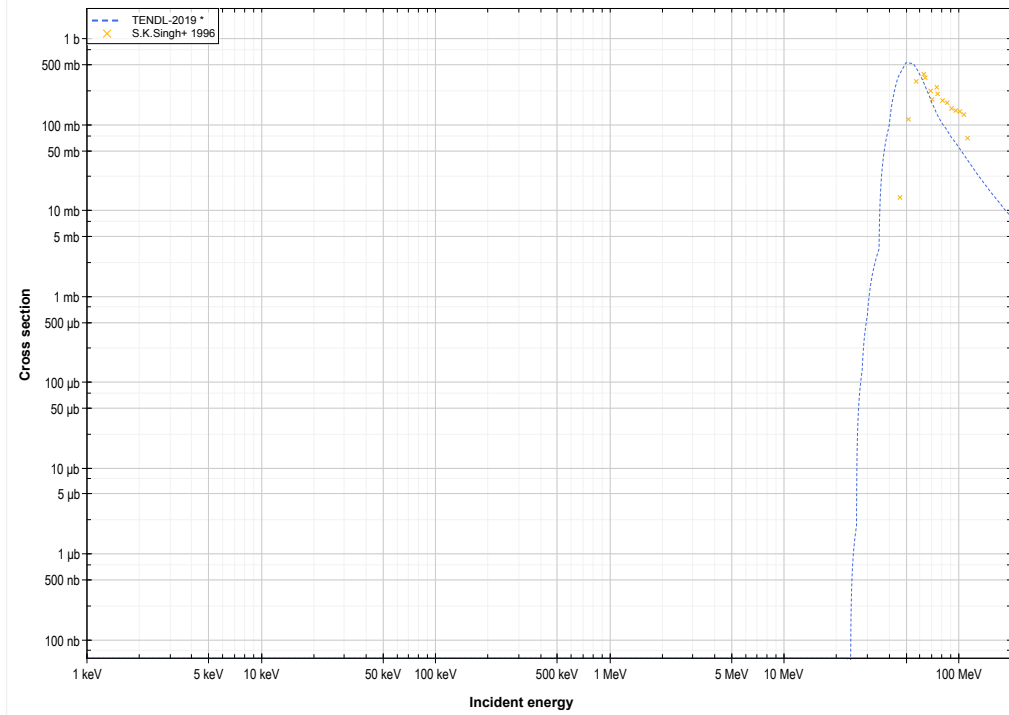
V51 ( \alpha, n+t ) or Cr51 production log-log
