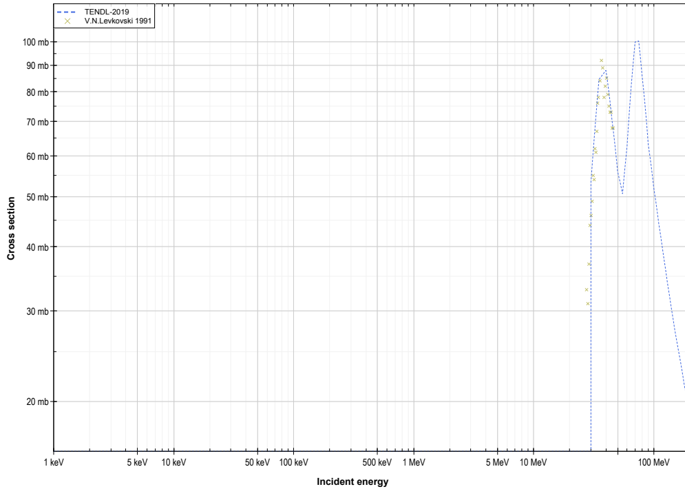
Y89 ( \alpha, 3n+2p ) or Y88 production log-log
