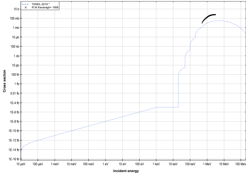
B11 (d,p) or B12 production log-log
