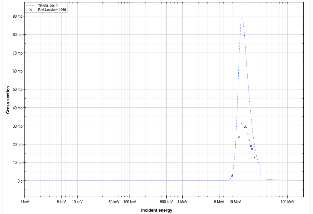
U234 (d,2n) or Np234 production lin-log
