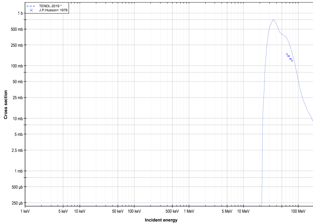
I127 (d,4n) or Xe125 production log-log
