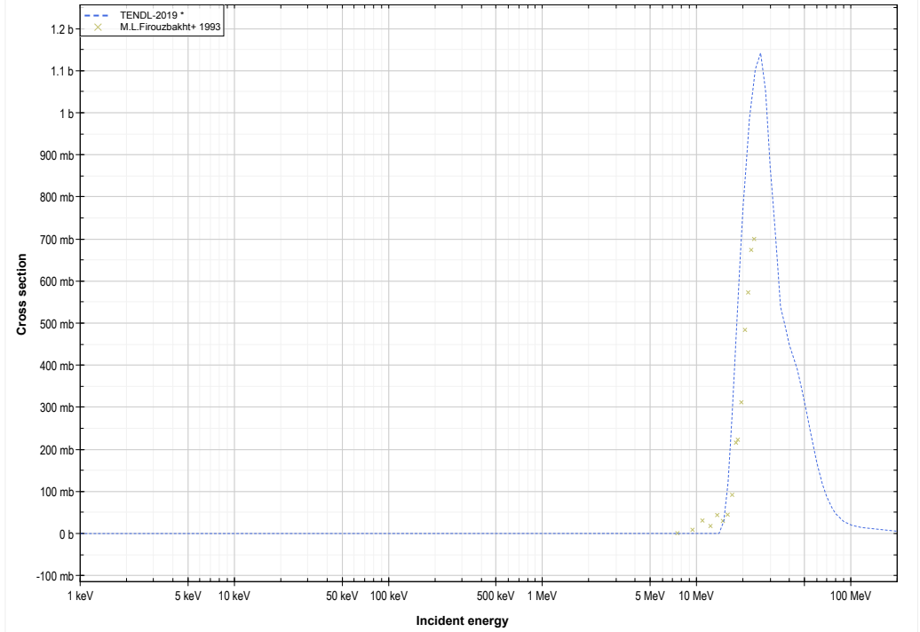
Te124 (d,3n) or I123 production lin-log
