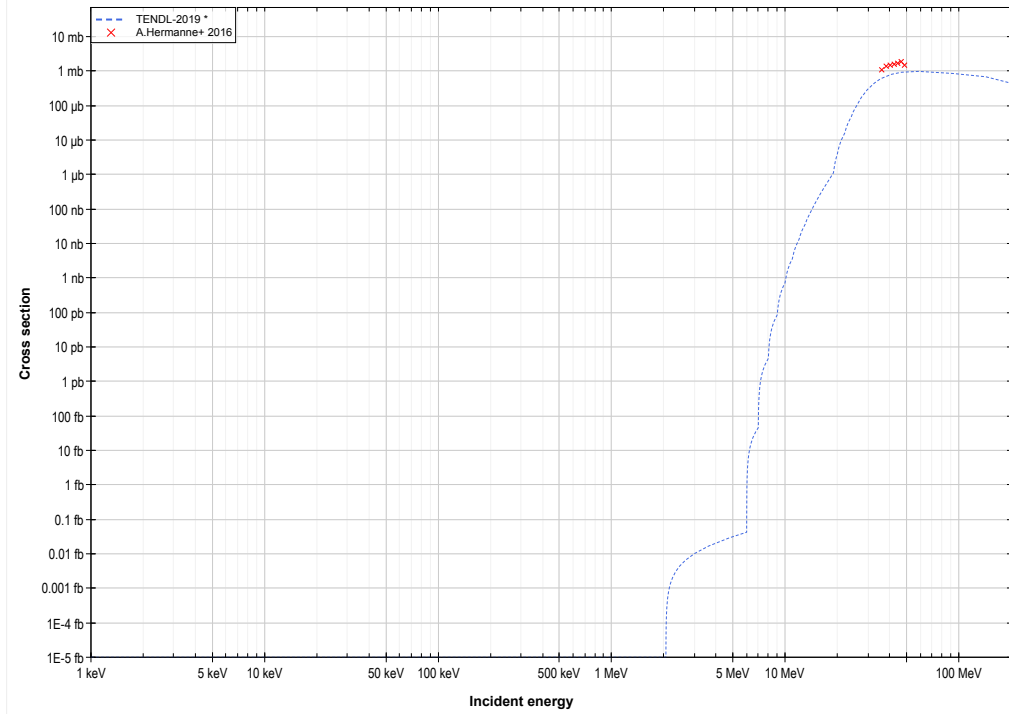
Pr141 (d,2p) or Ce141 production log-log
