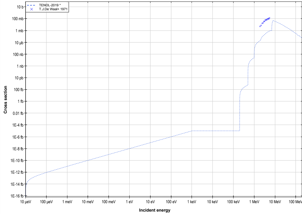
Ca48 (d,p) or Ca49 production log-log
