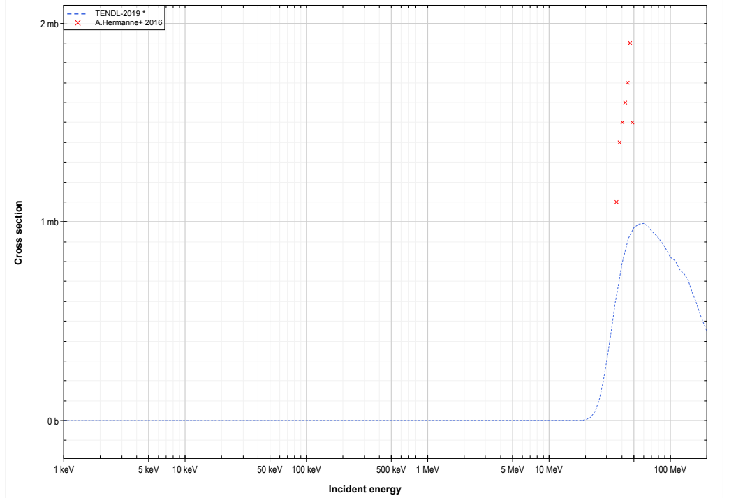
Pr141 (d,2p) or Ce141 production lin-log
