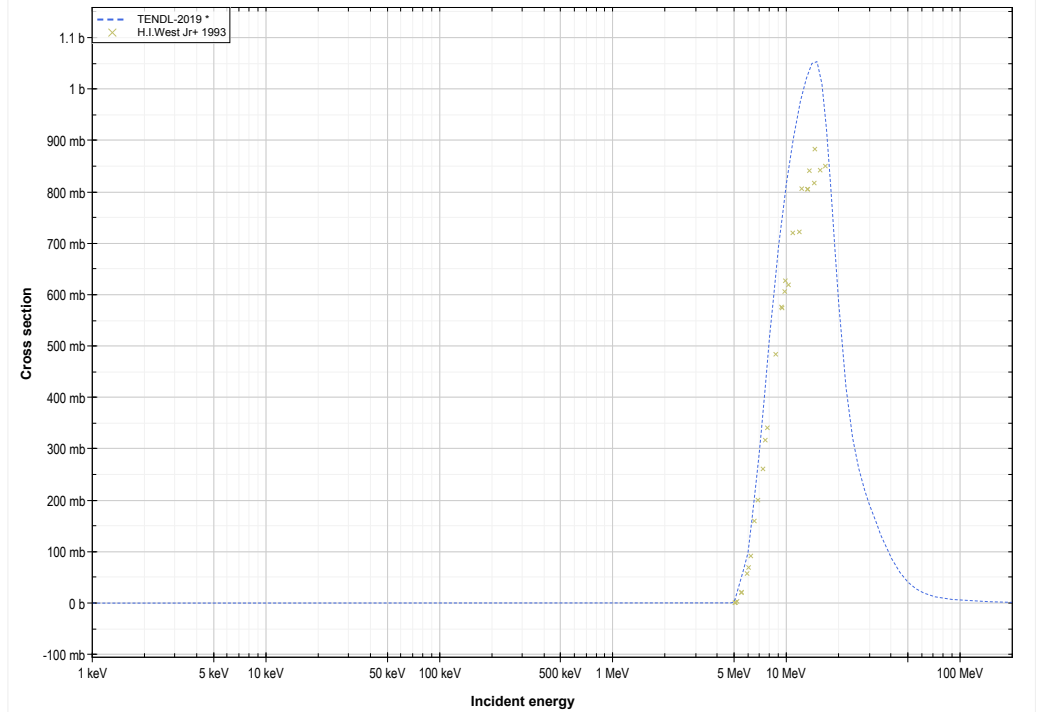
Br79 (d,2n) or Kr79 production lin-log
