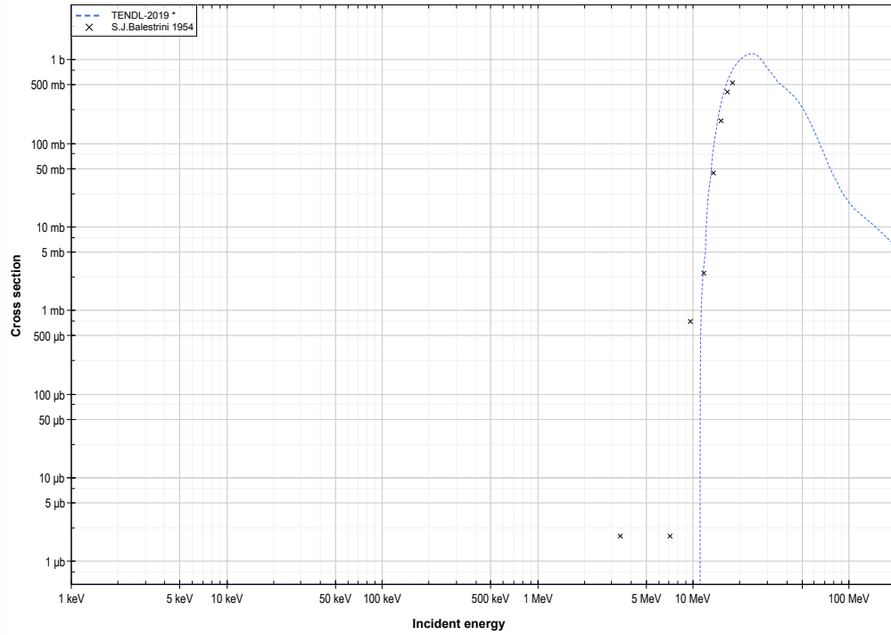
I127 (d,3n) or Xe126 production log-log
