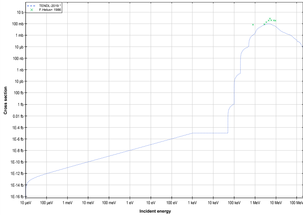
Ne22 (d,p) or Ne23 production log-log
