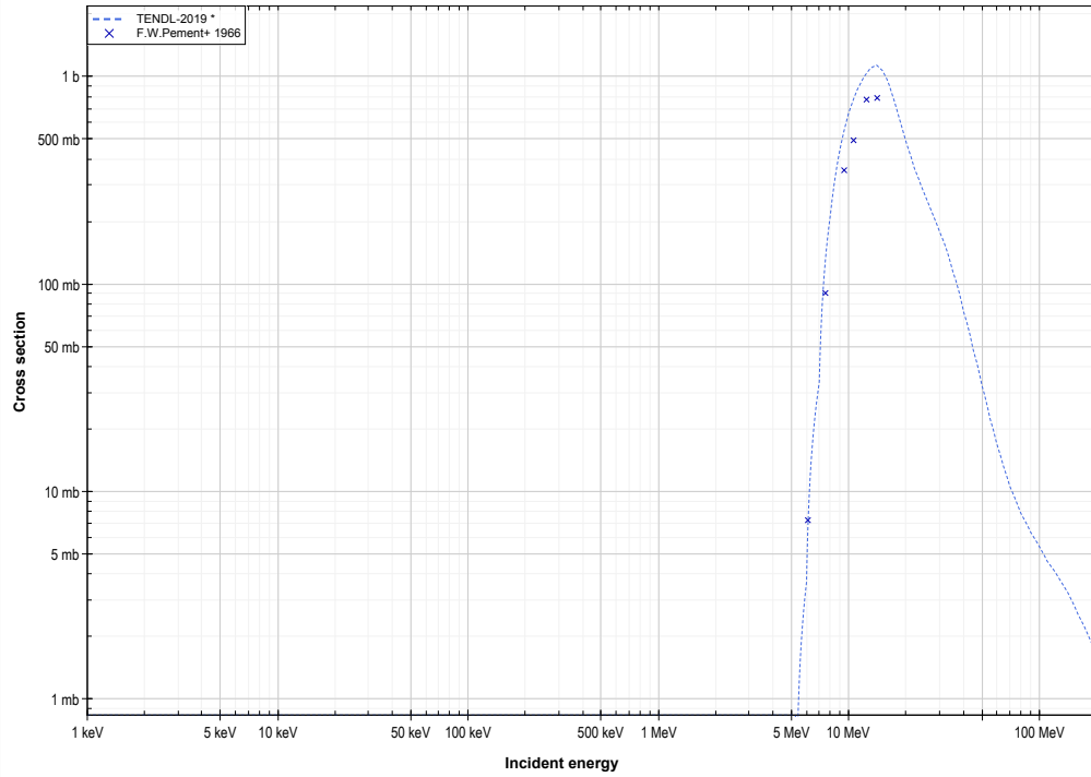
Te126 (d,2n) or I126 production log-log
