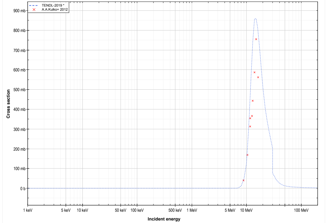
Pt194 (d,2n) or Au194 production lin-log
