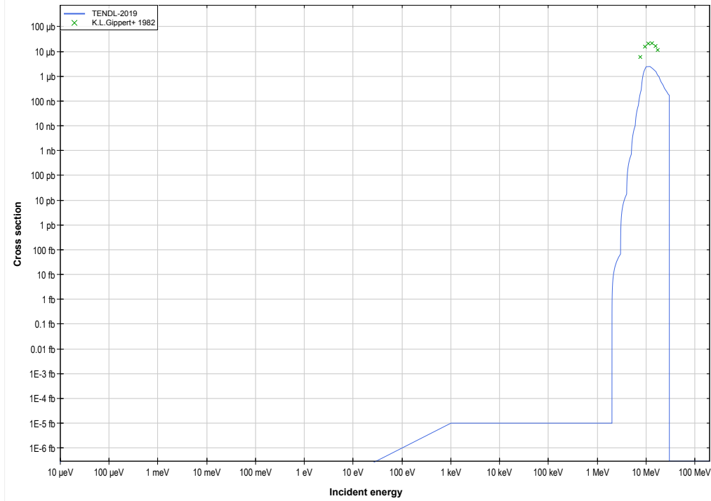
Sm154 (d, \gamma ) or Eu156 production log-log
