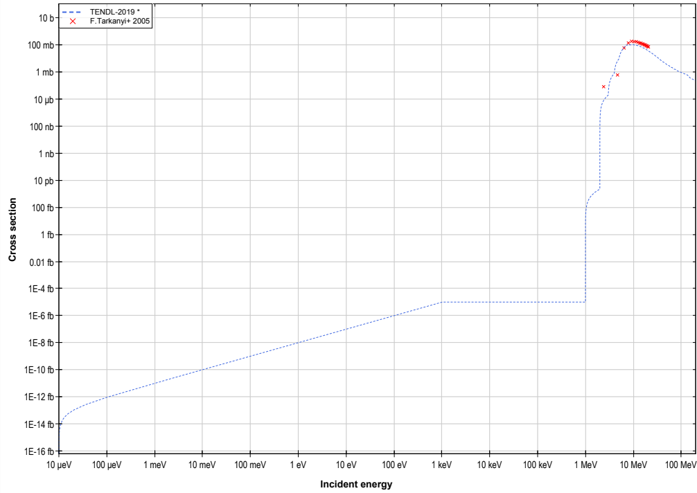
Cd114 (d,p) or Cd115 production log-log
