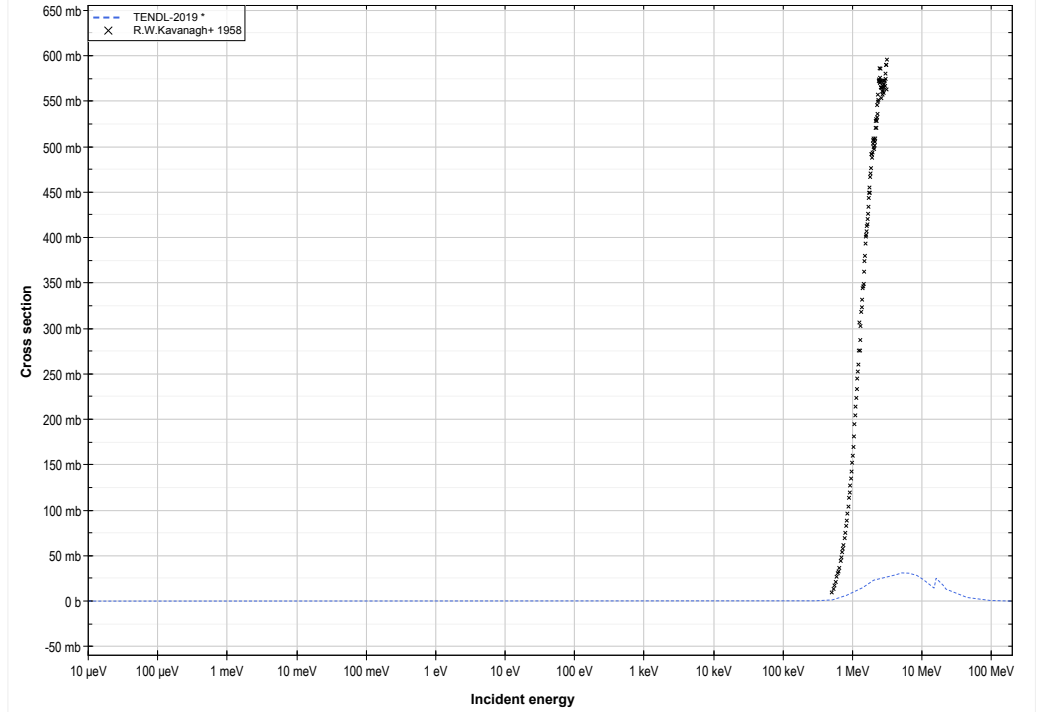
B11 (d,p) or B12 production lin-log
