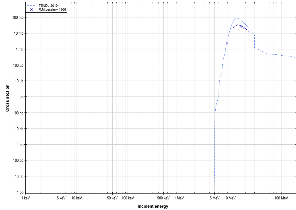
U234 (d,2n) or Np234 production log-log
