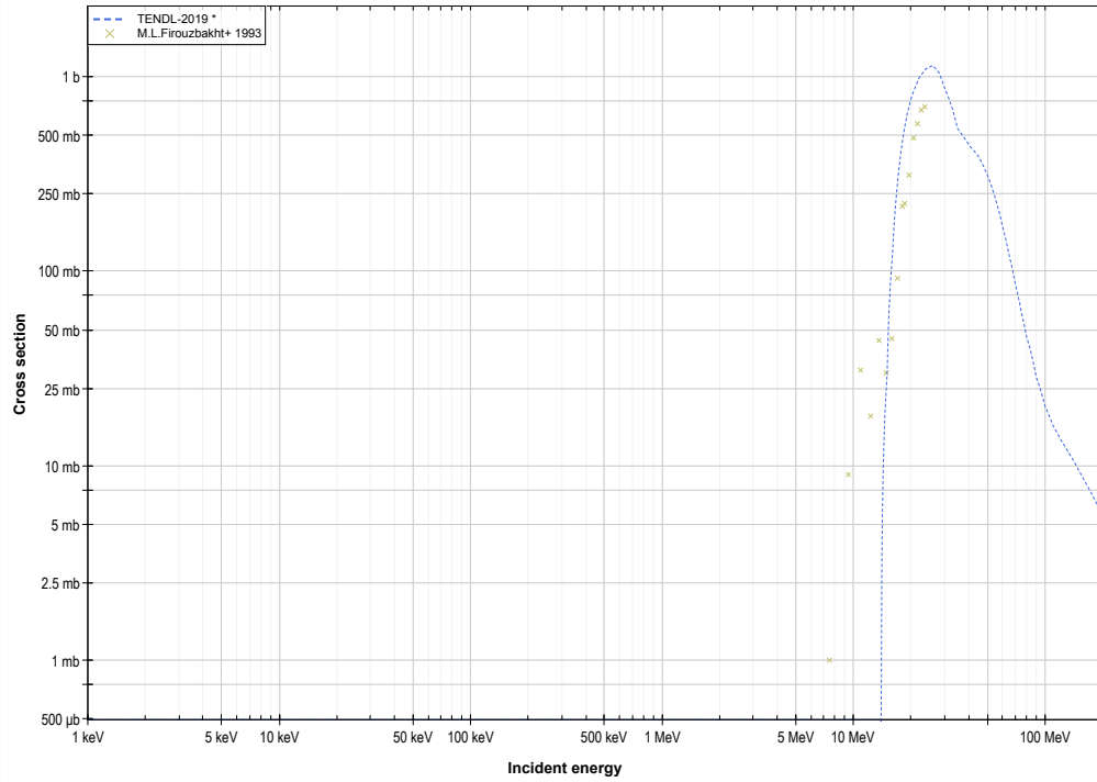
Te124 (d,3n) or I123 production log-log
