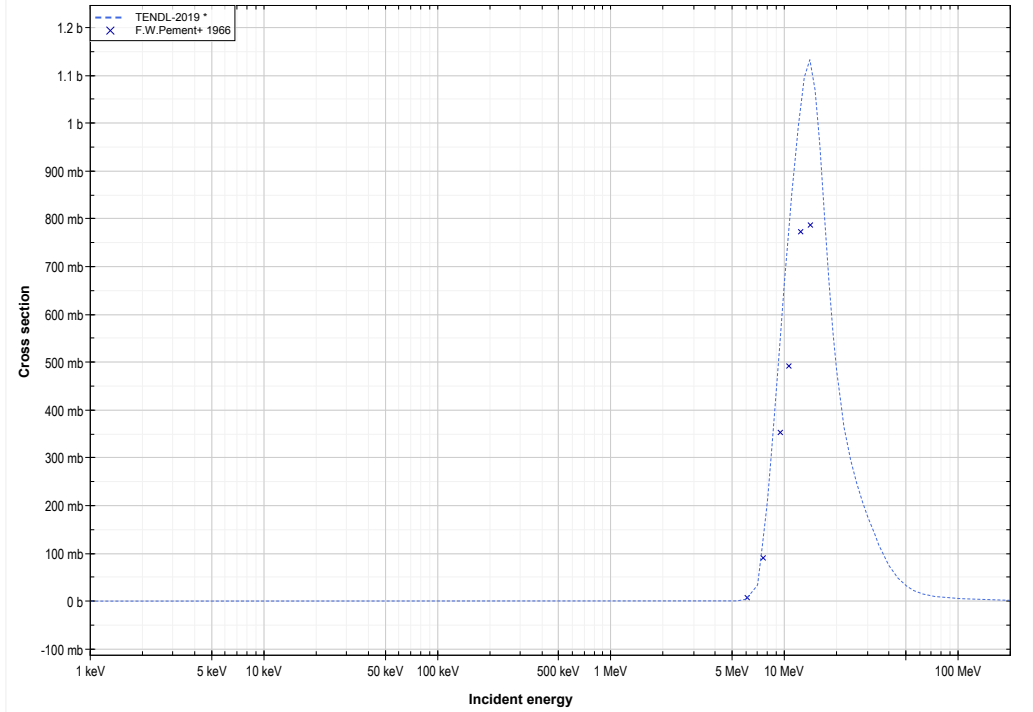
Te126 (d,2n) or I126 production lin-log
