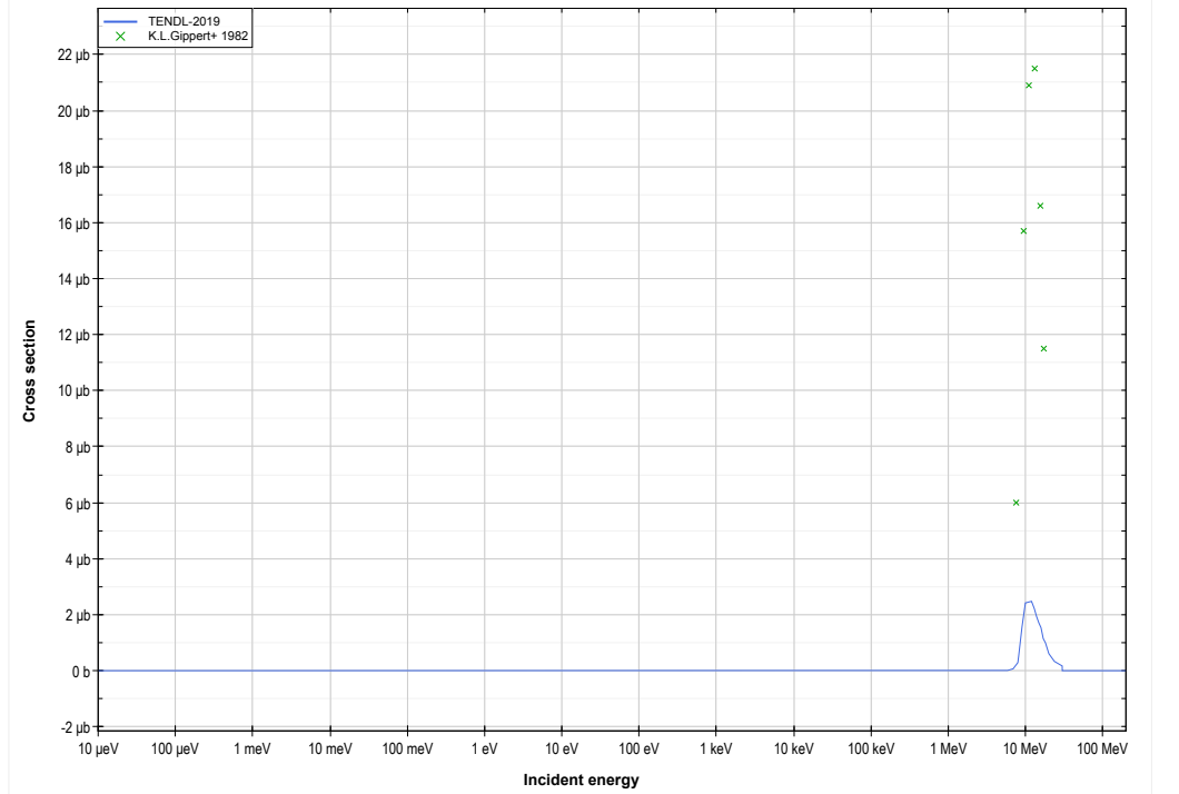
Sm154 (d, \gamma ) or Eu156 production lin-log
