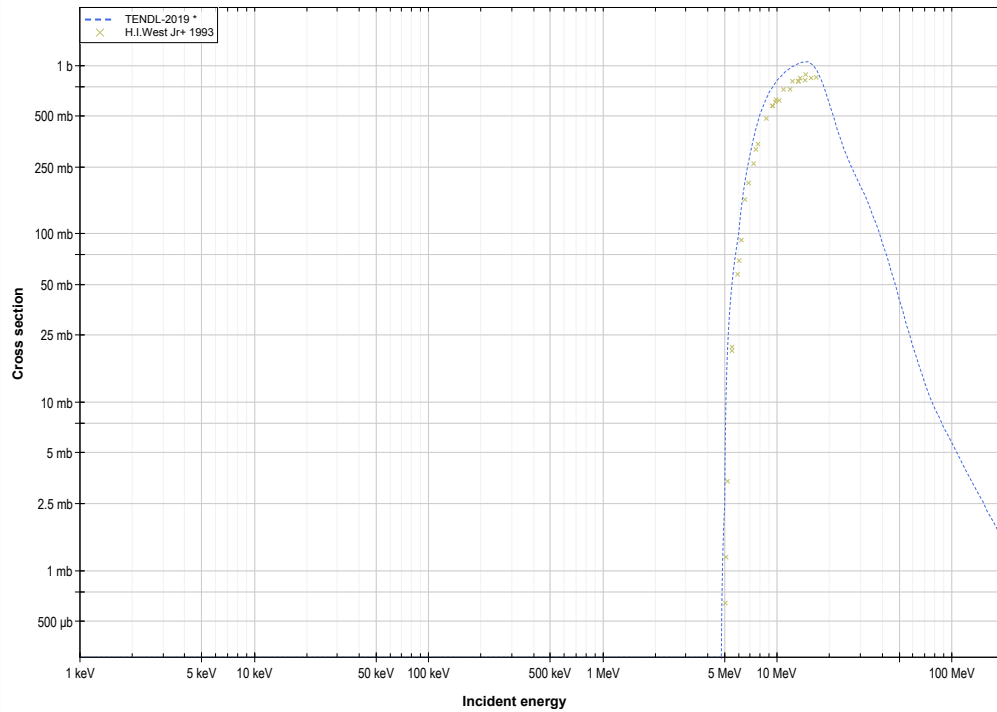
Br79 (d,2n) or Kr79 production log-log
