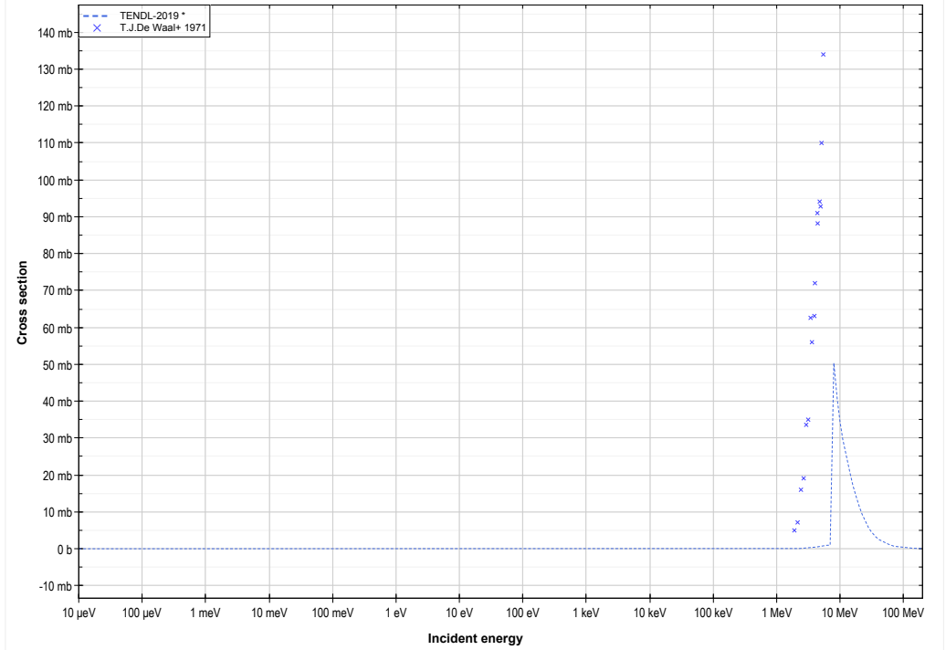
Ca48 (d,p) or Ca49 production lin-log
