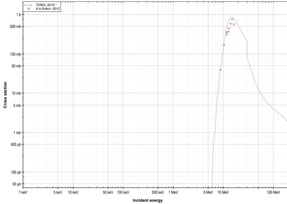
Pt194 (d,2n) or Au194 production log-log
