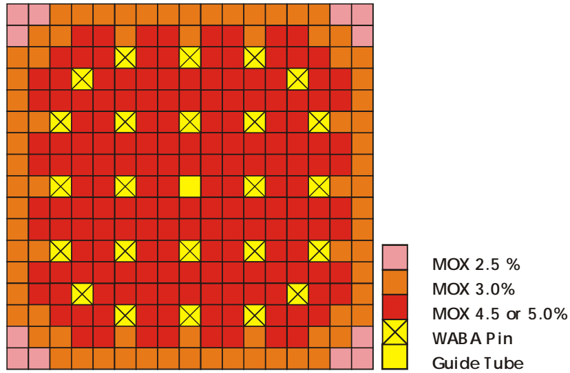
Figure 3. MOX fuel assembly with 24 WABA pins
