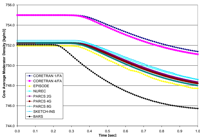
Figure 15. Part IV, transient core average moderator density
