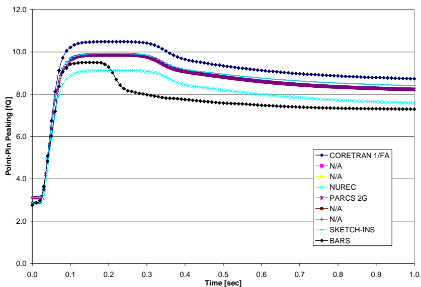
Figure 13. Part IV, transient point pin peaking
