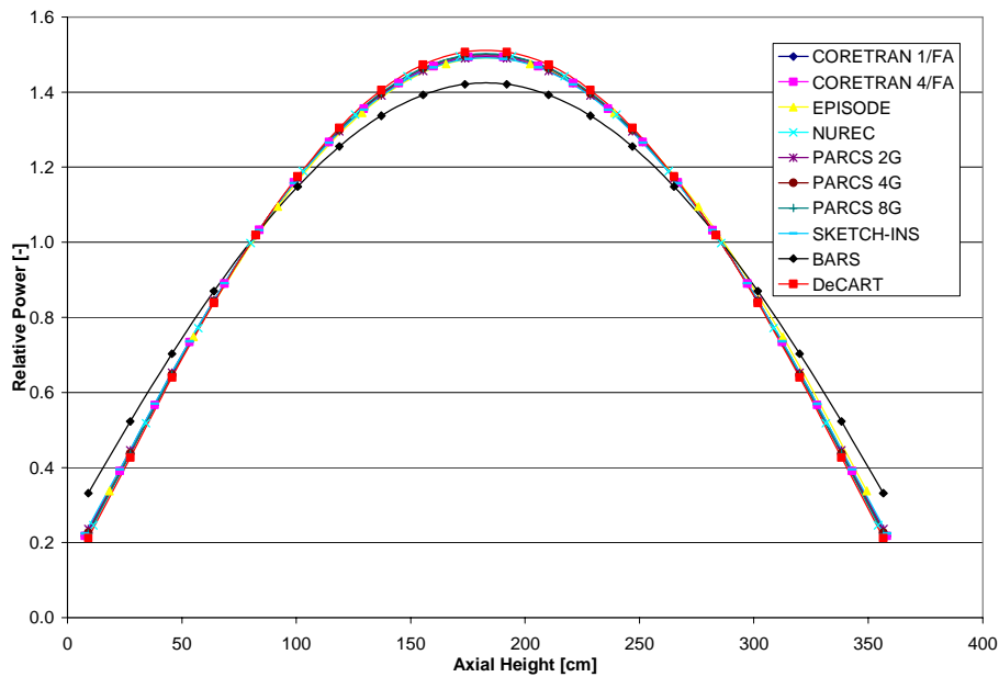
Figure 8. Part III, axial power distribution
