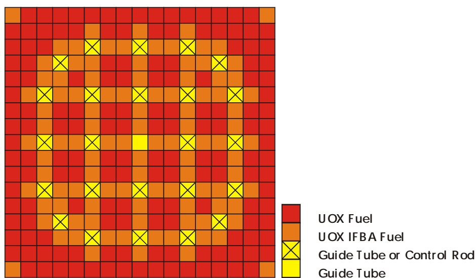
Figure 2. UO_2 fuel assembly with 104 IFBA pins
