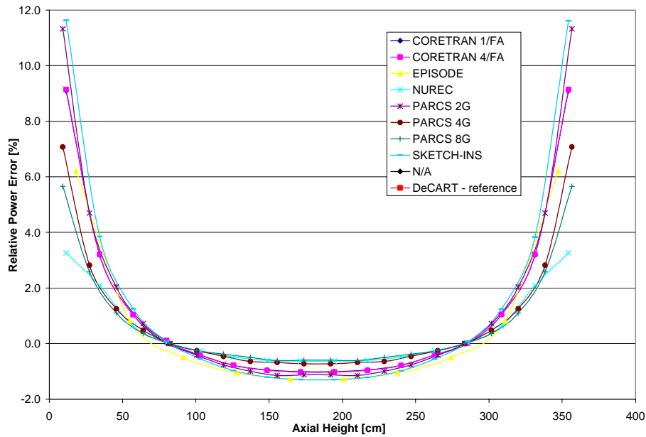
Figure 9. Part III, axial power distribution error
