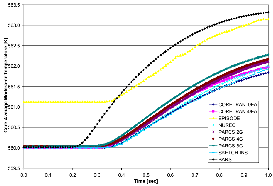
Figure 16. Part IV, transient core average moderator temperature
