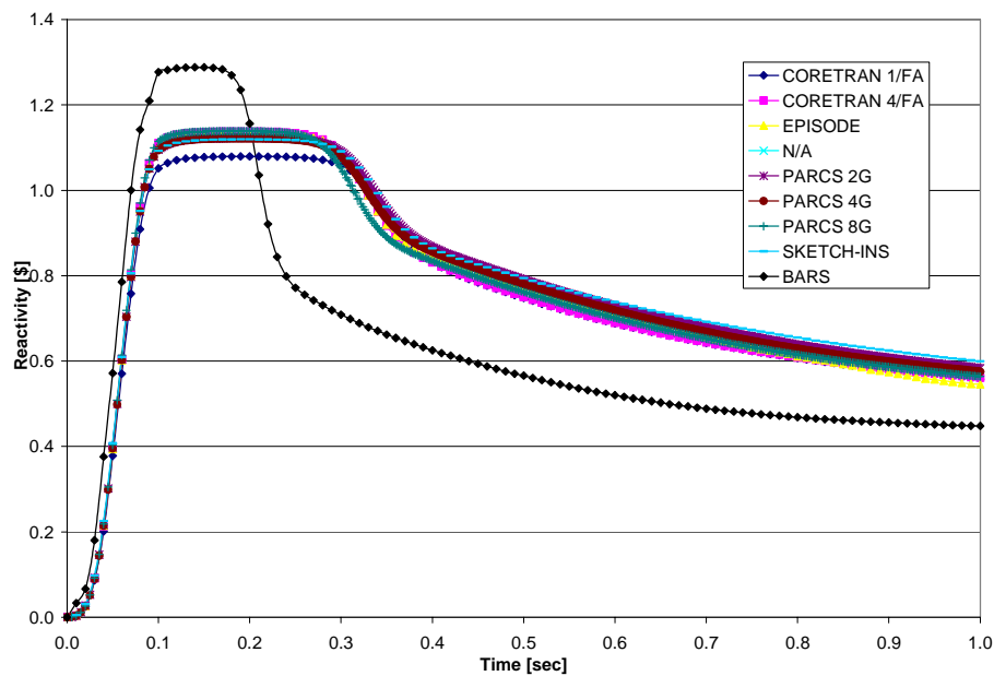
Figure 11. Part IV, transient reactivity
